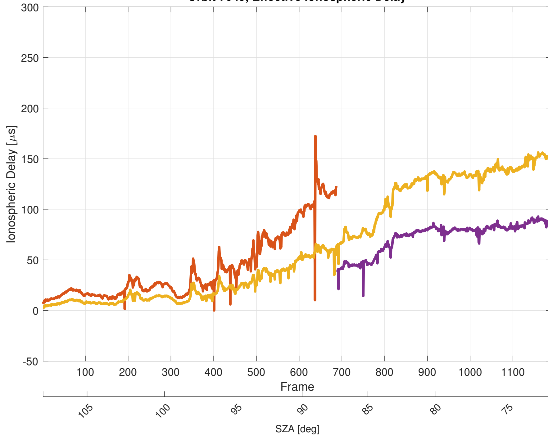
Orbit 7049, Effective Ionospheric Delay
