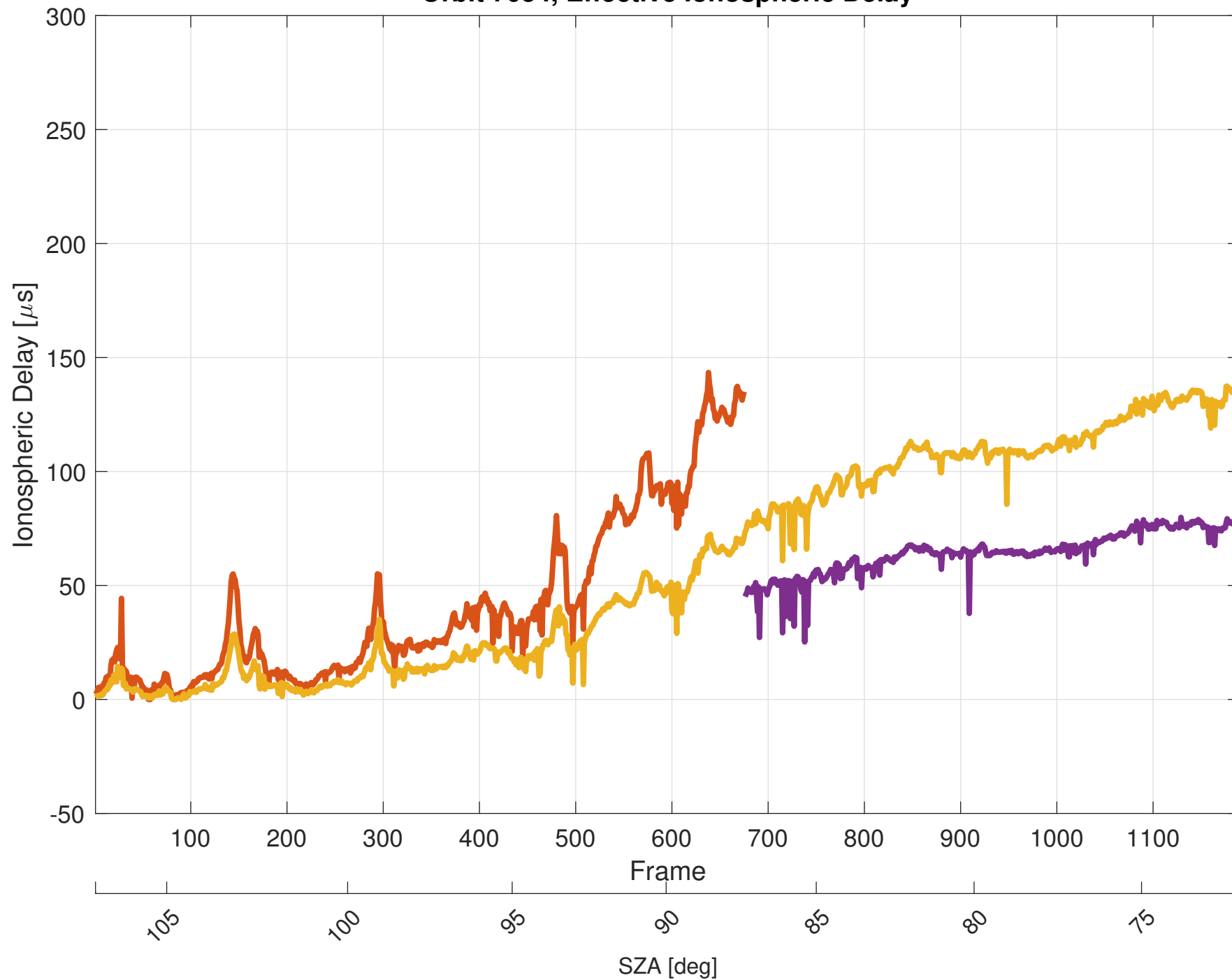
Orbit 7054, Effective Ionospheric Delay
