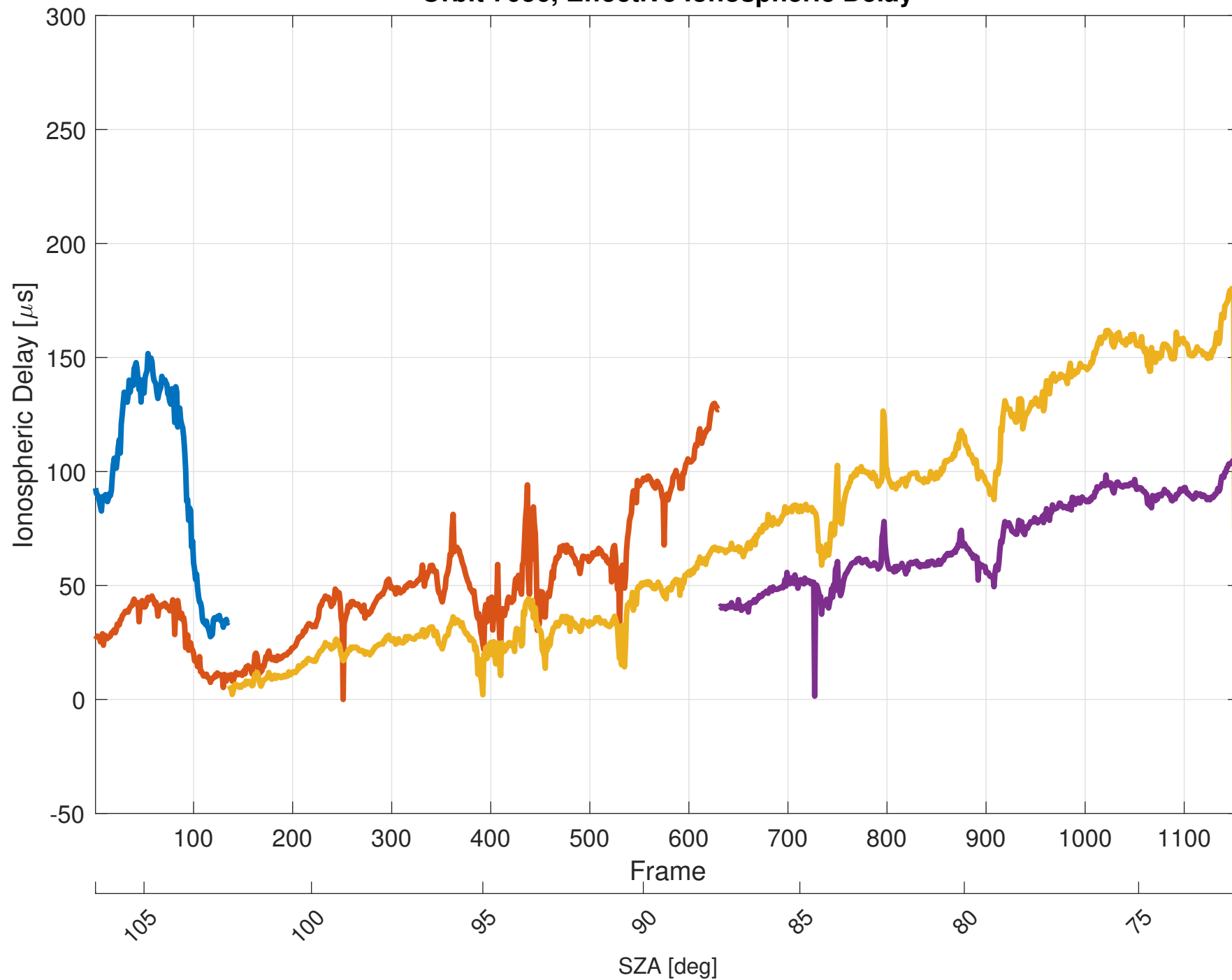
Orbit 7056, Effective Ionospheric Delay
