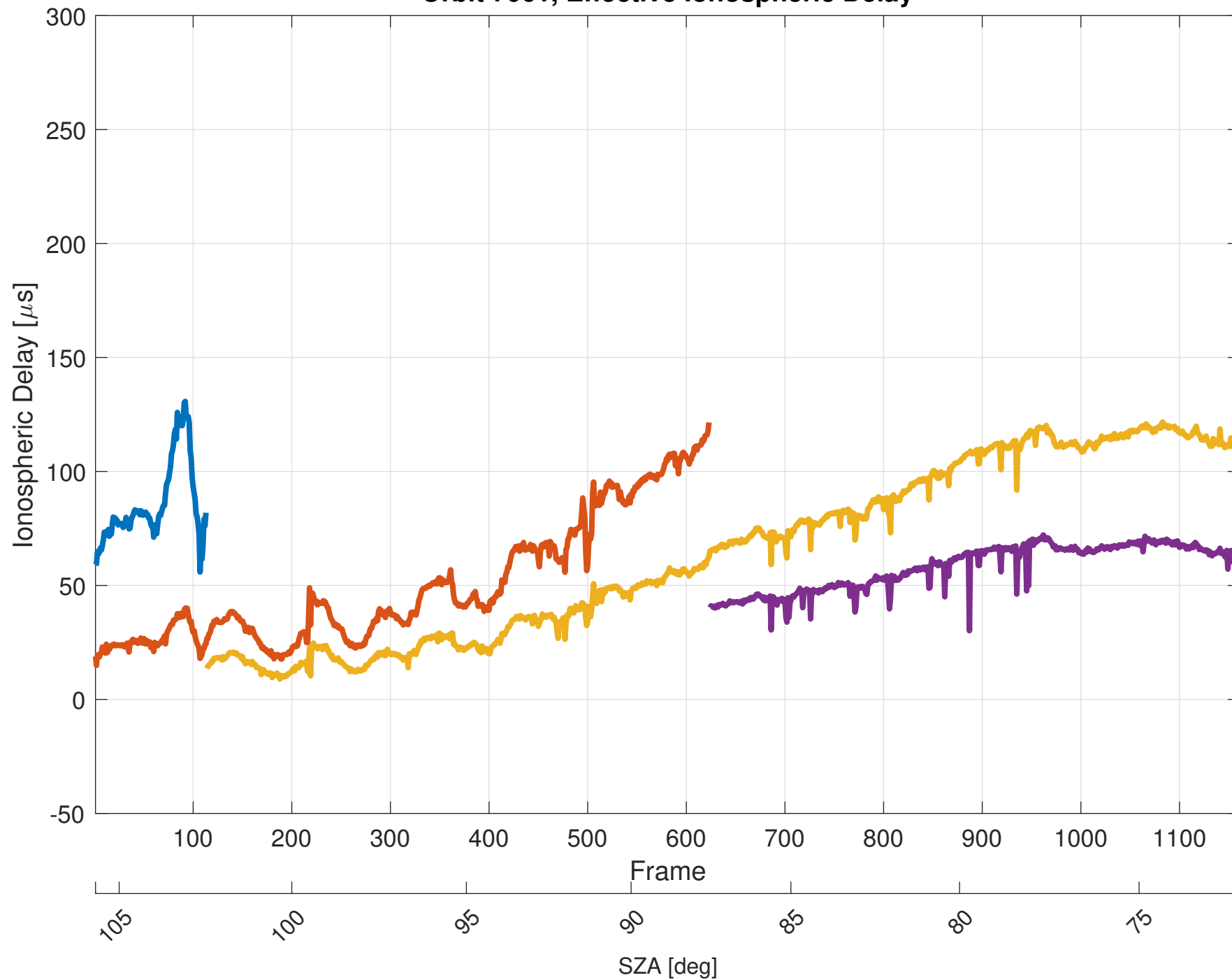
Orbit 7061, Effective Ionospheric Delay
