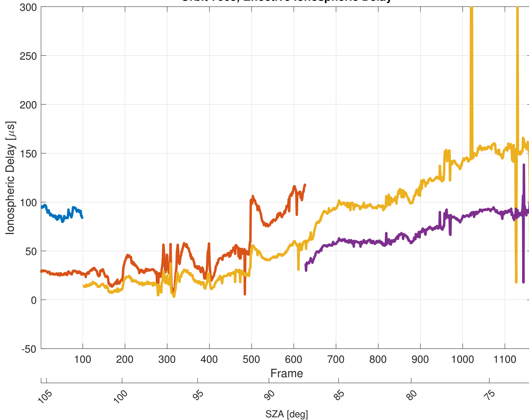
Orbit 7063, Effective Ionospheric Delay
