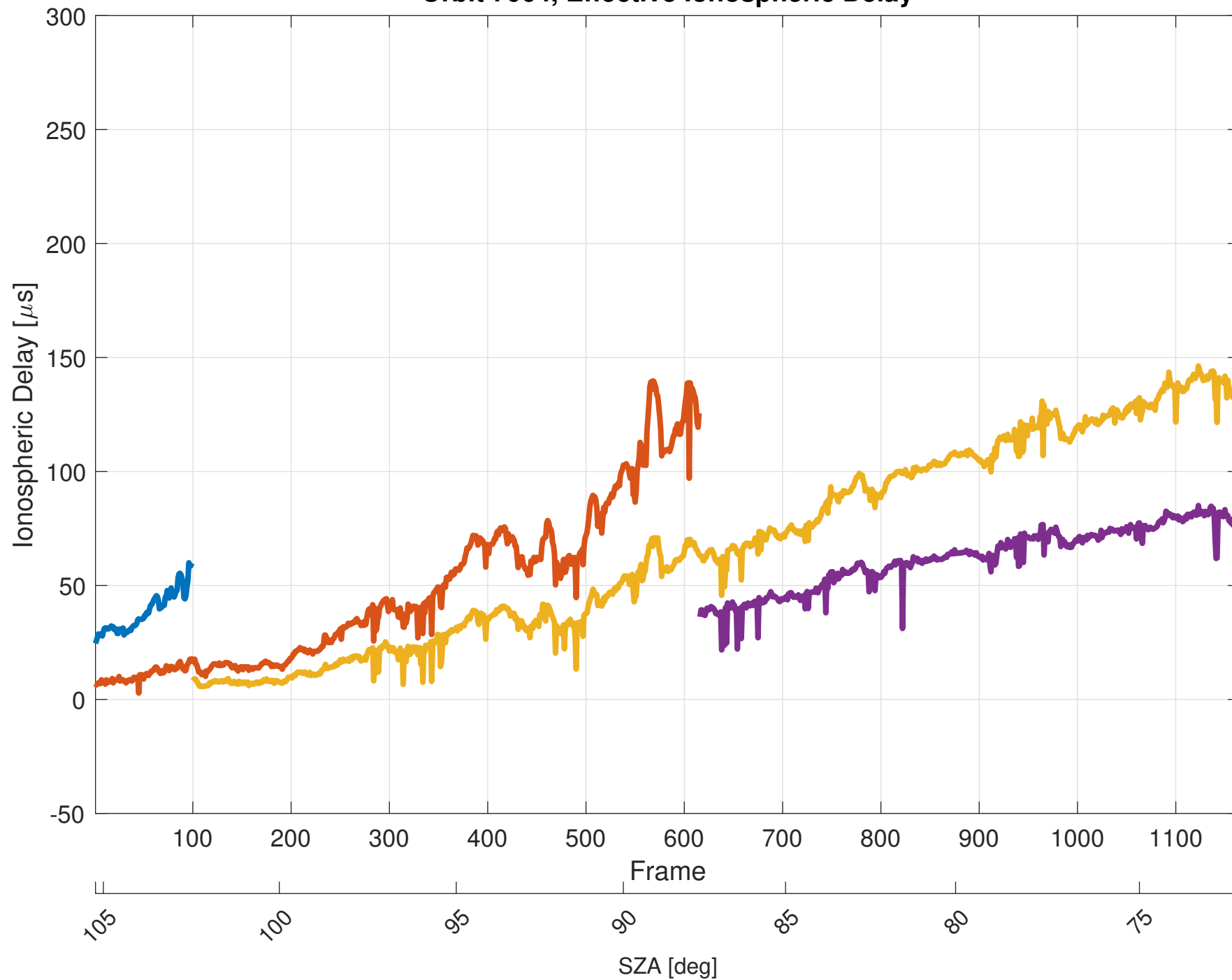
Orbit 7064, Effective Ionospheric Delay
