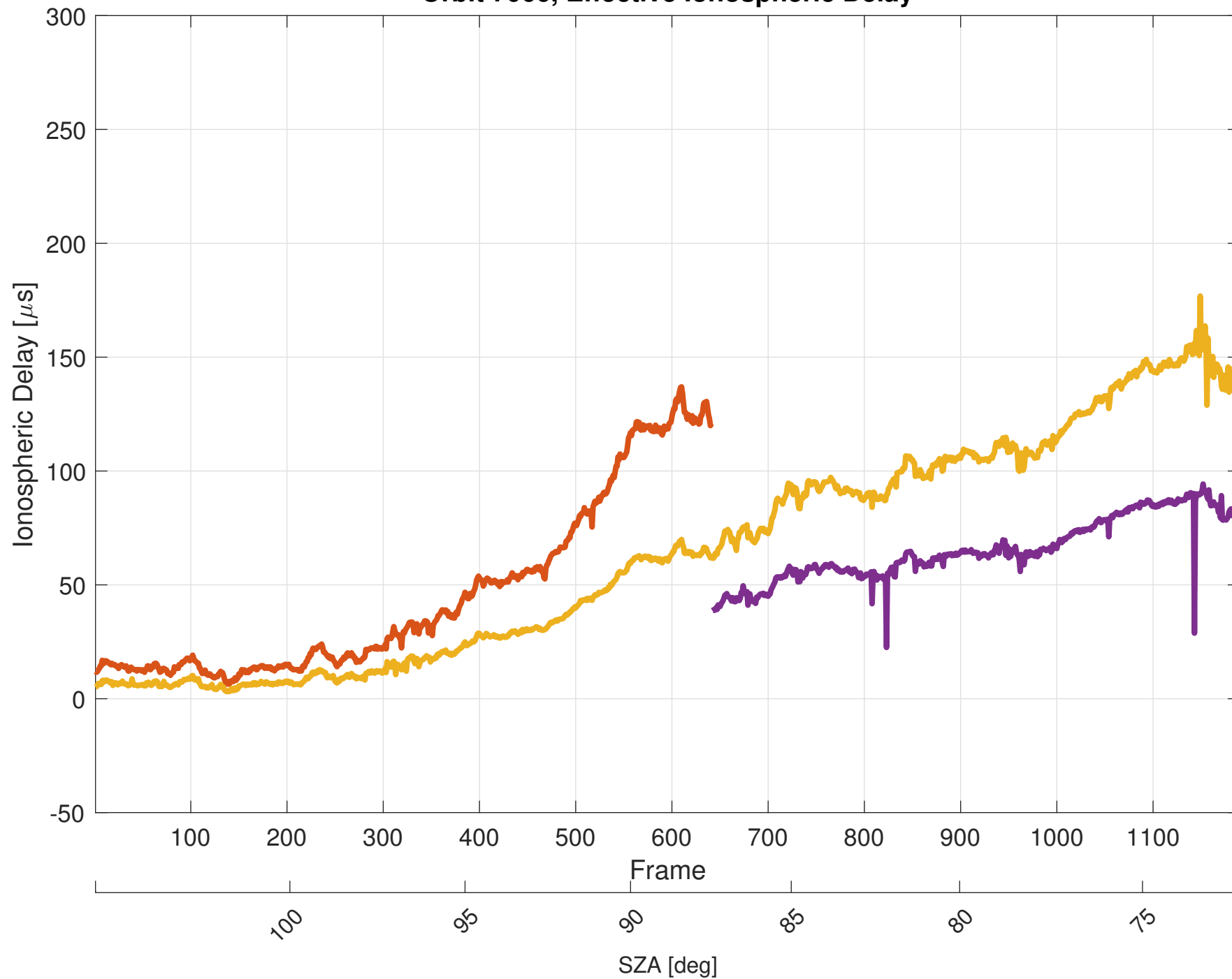
Orbit 7066, Effective Ionospheric Delay
