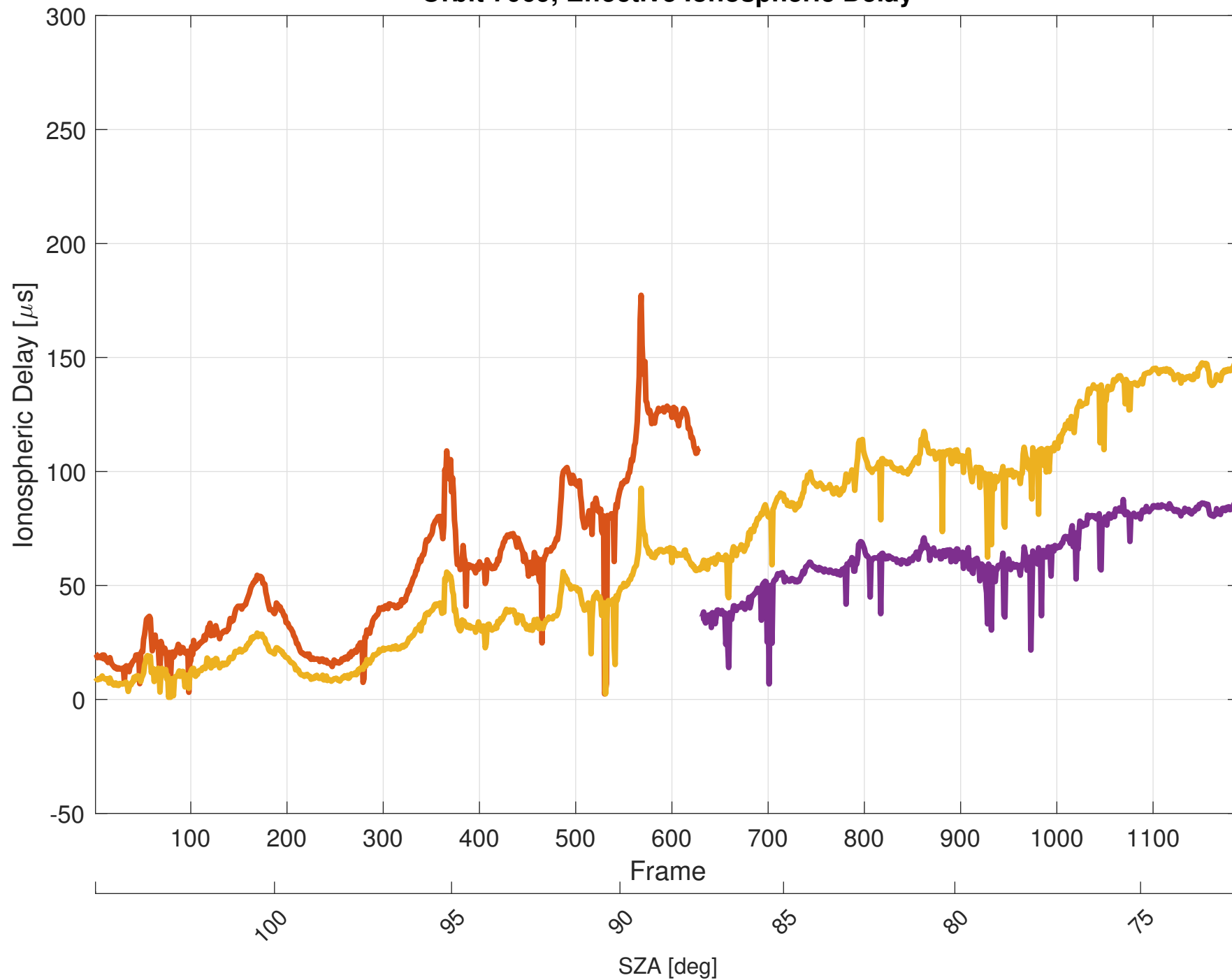
Orbit 7069, Effective Ionospheric Delay
