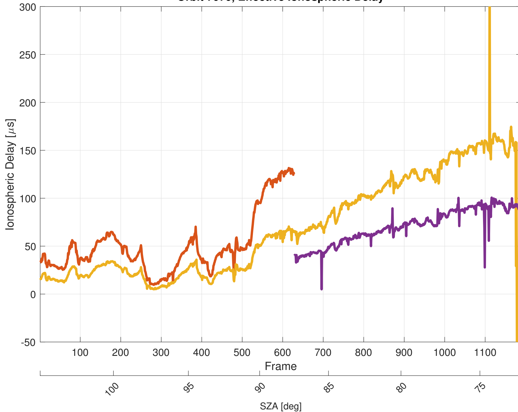
Orbit 7070, Effective Ionospheric Delay
