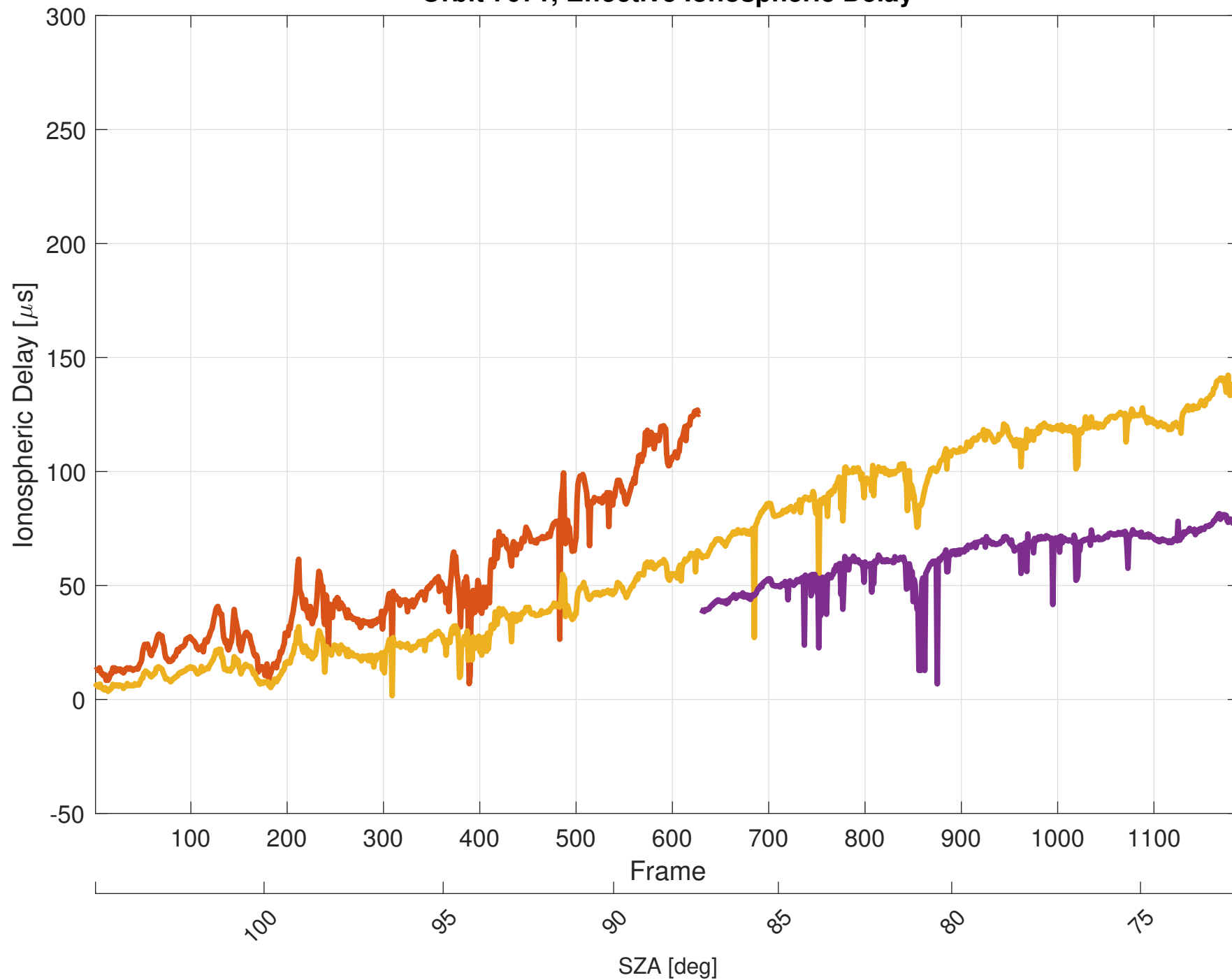
Orbit 7071, Effective Ionospheric Delay
