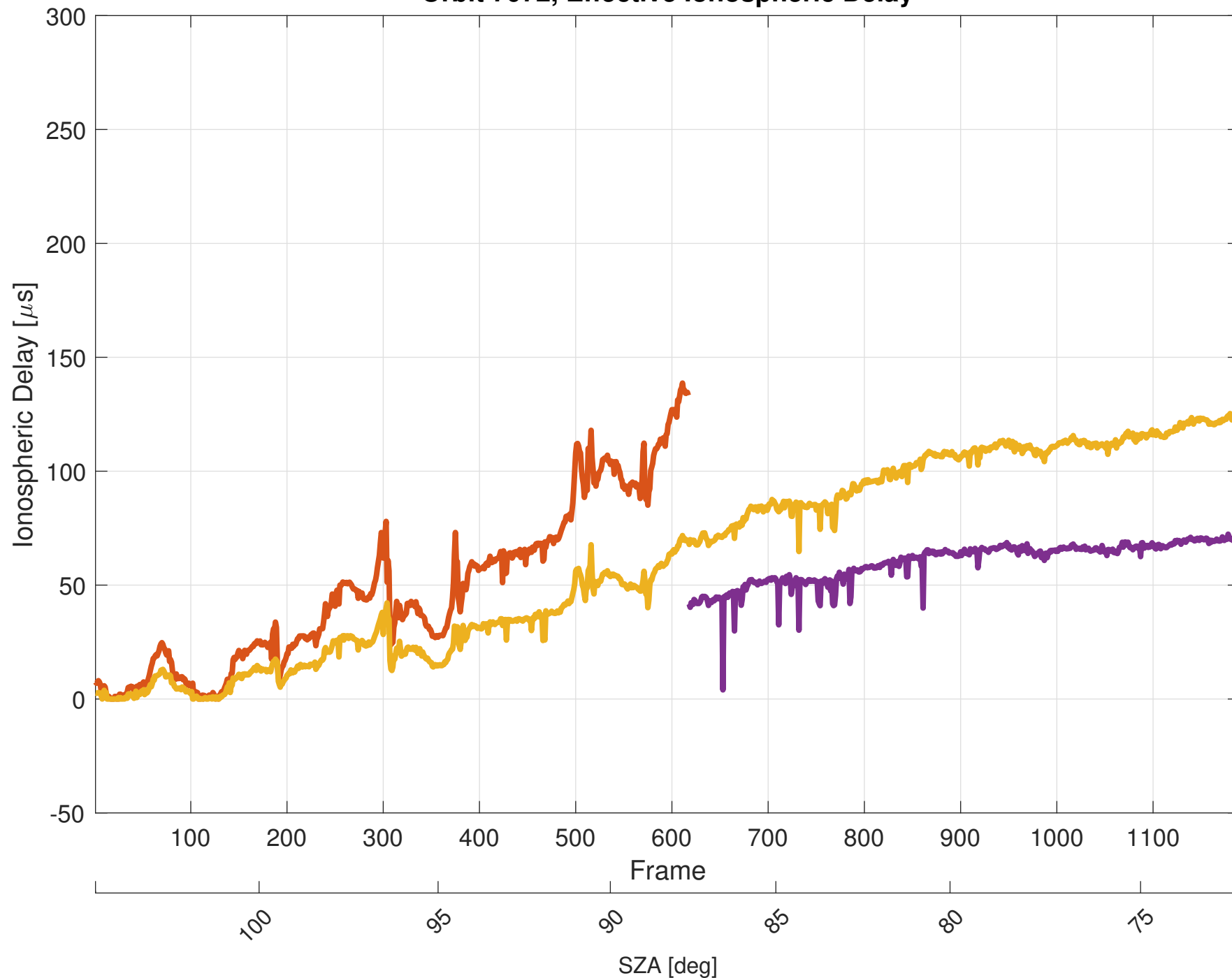
Orbit 7072, Effective Ionospheric Delay
