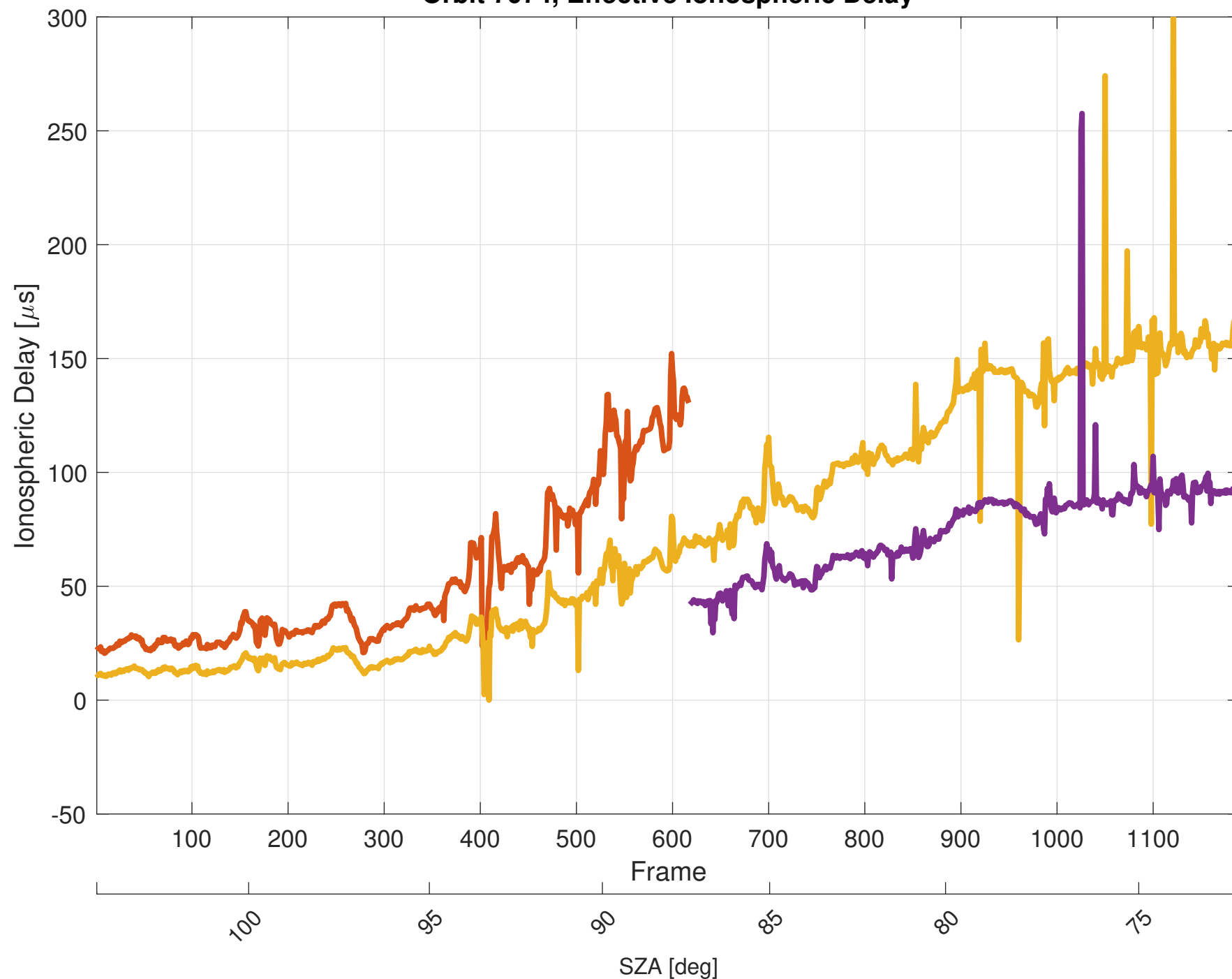
Orbit 7074, Effective Ionospheric Delay
