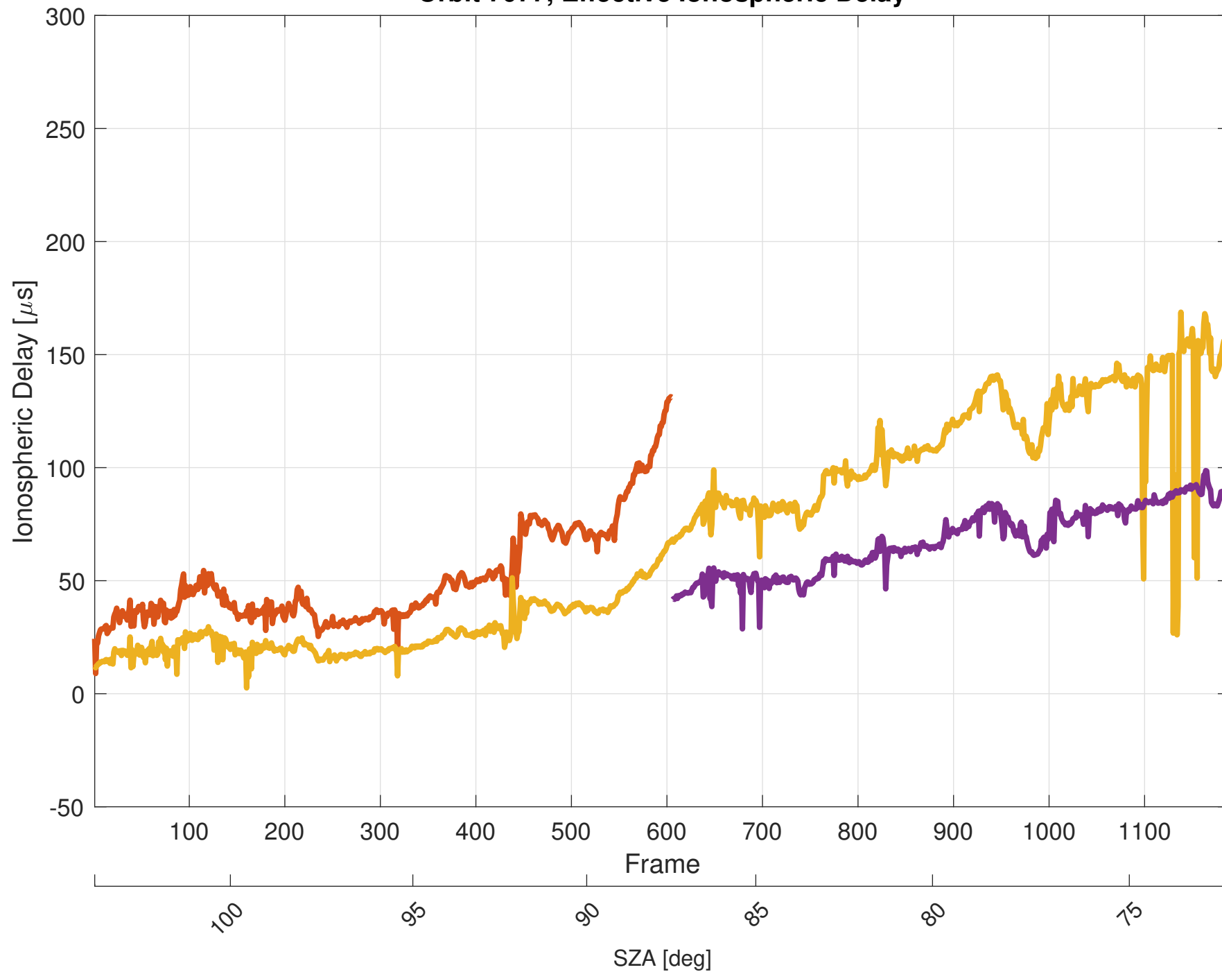
Orbit 7077, Effective Ionospheric Delay
