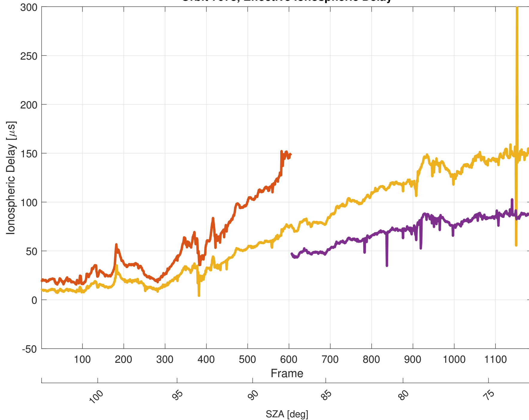
Orbit 7078, Effective Ionospheric Delay
