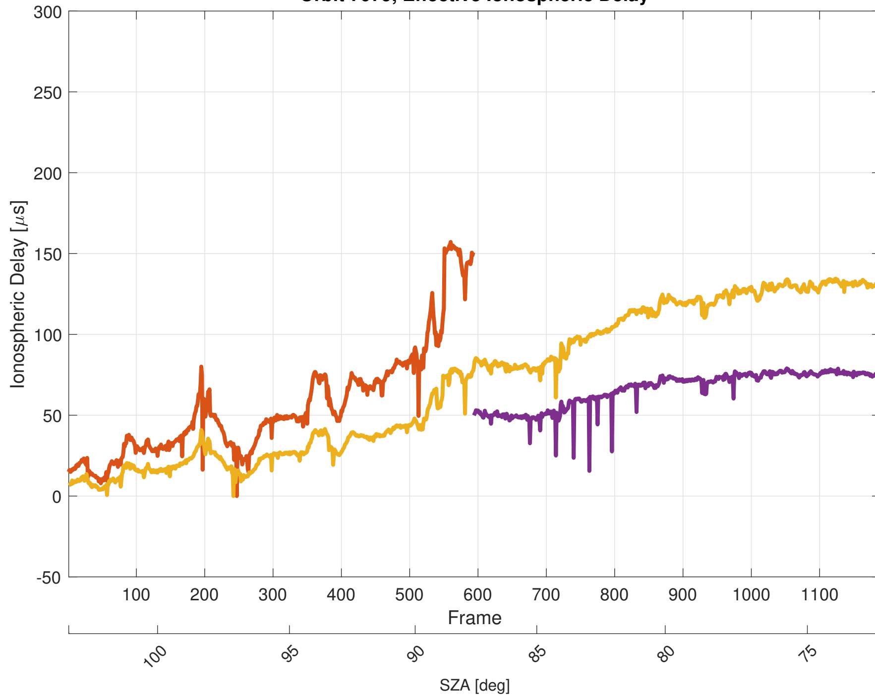
Orbit 7079, Effective Ionospheric Delay
