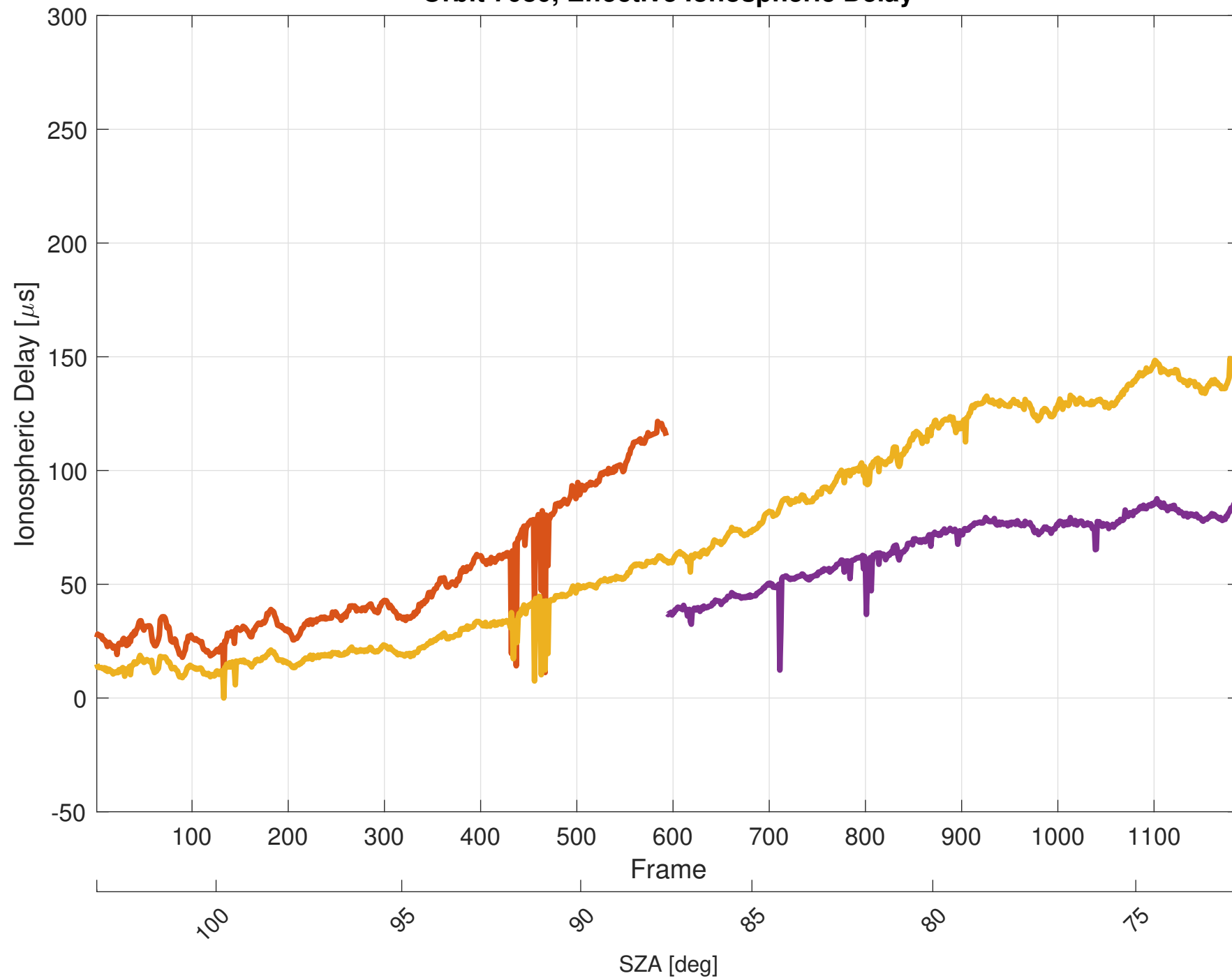
Orbit 7080, Effective Ionospheric Delay
