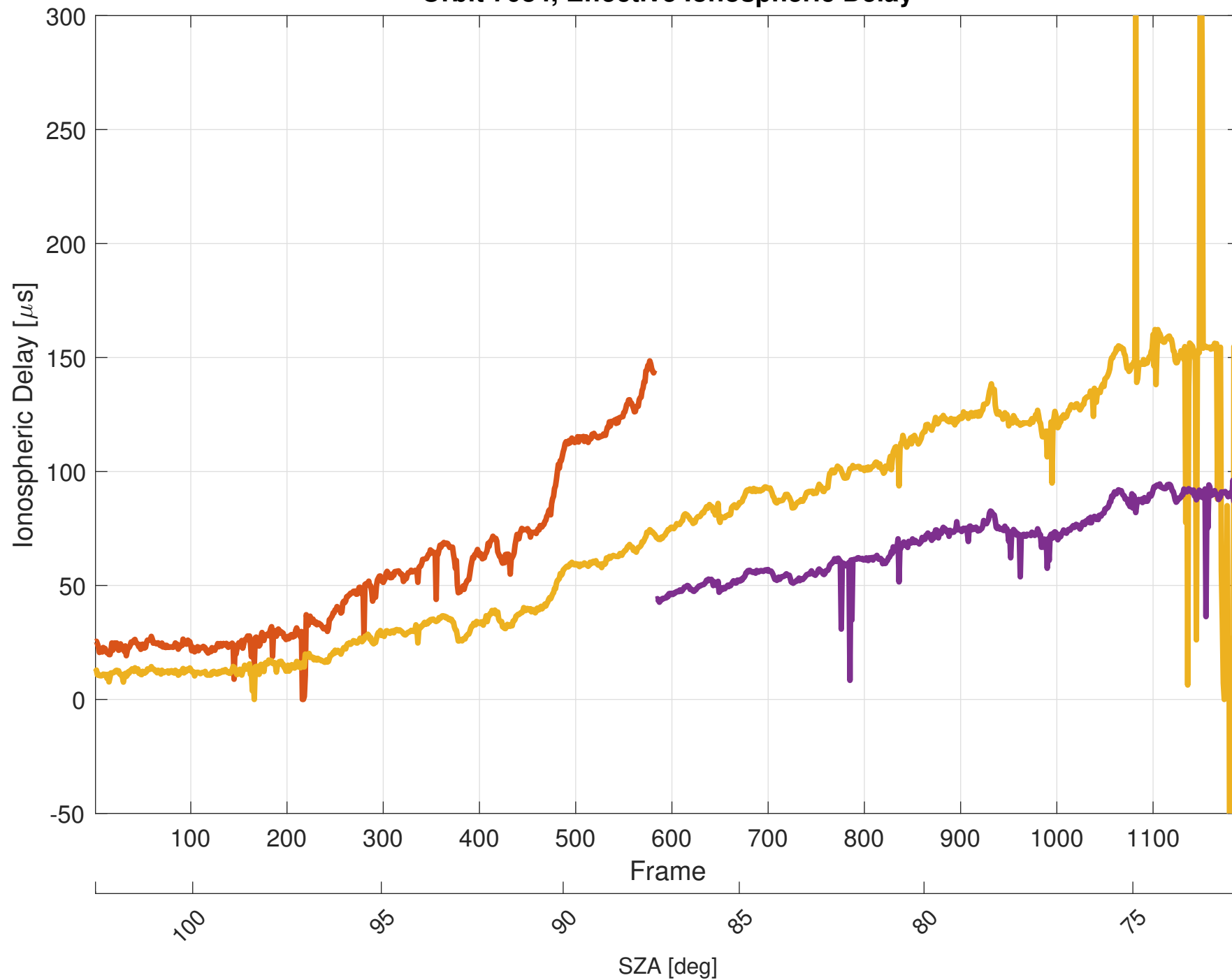
Orbit 7084, Effective Ionospheric Delay
