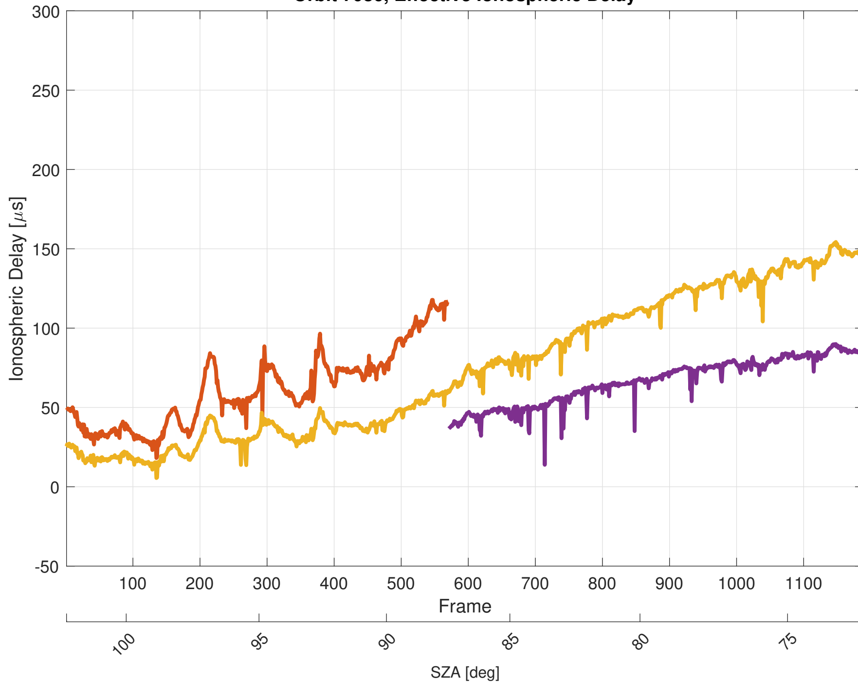
Orbit 7086, Effective Ionospheric Delay
