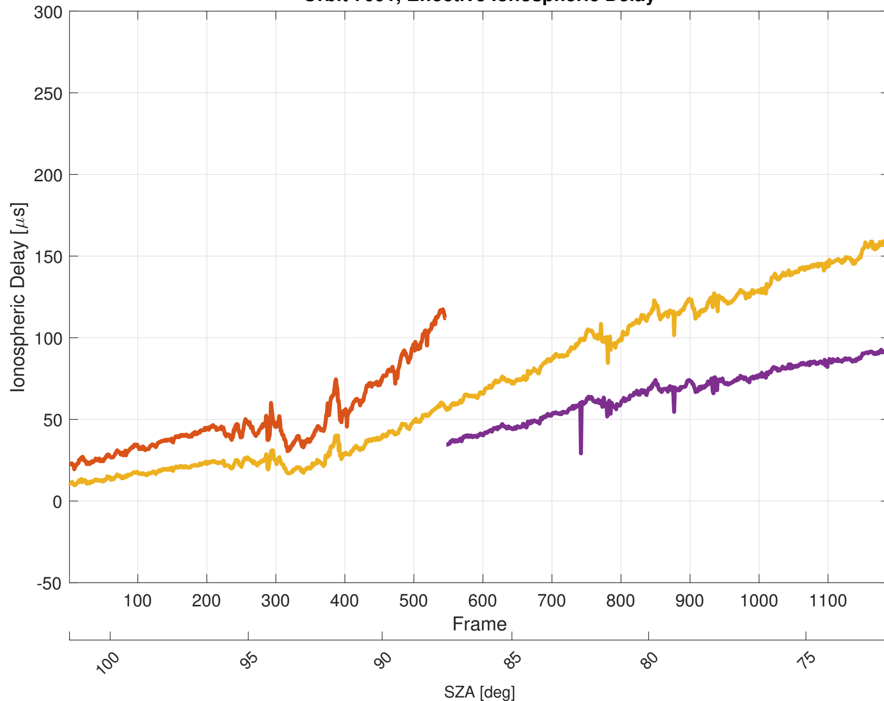
Orbit 7091, Effective Ionospheric Delay
