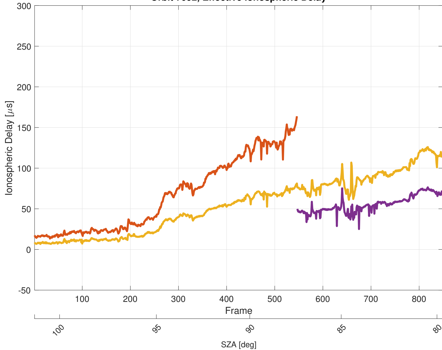
Orbit 7092, Effective Ionospheric Delay
