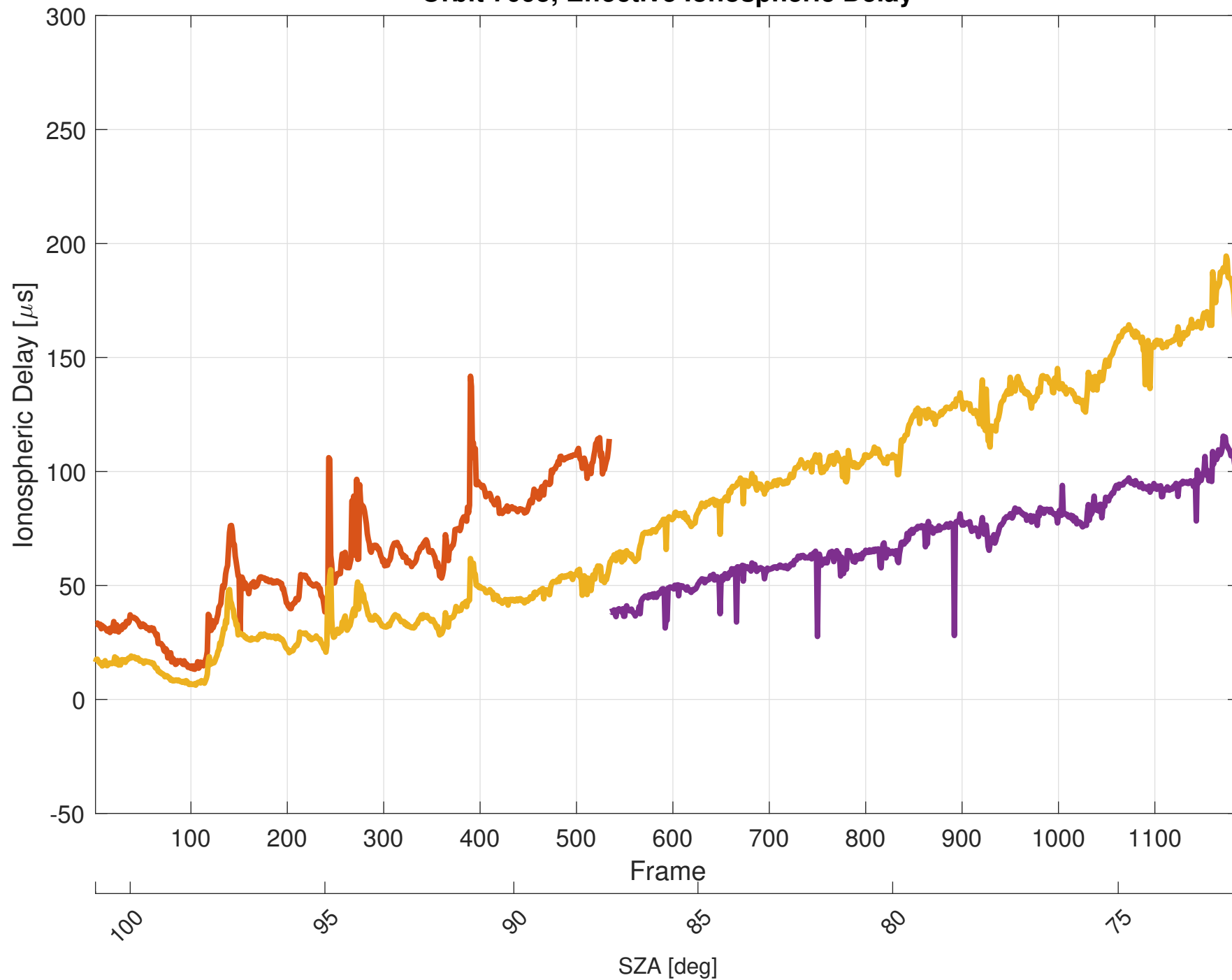
Orbit 7095, Effective Ionospheric Delay
