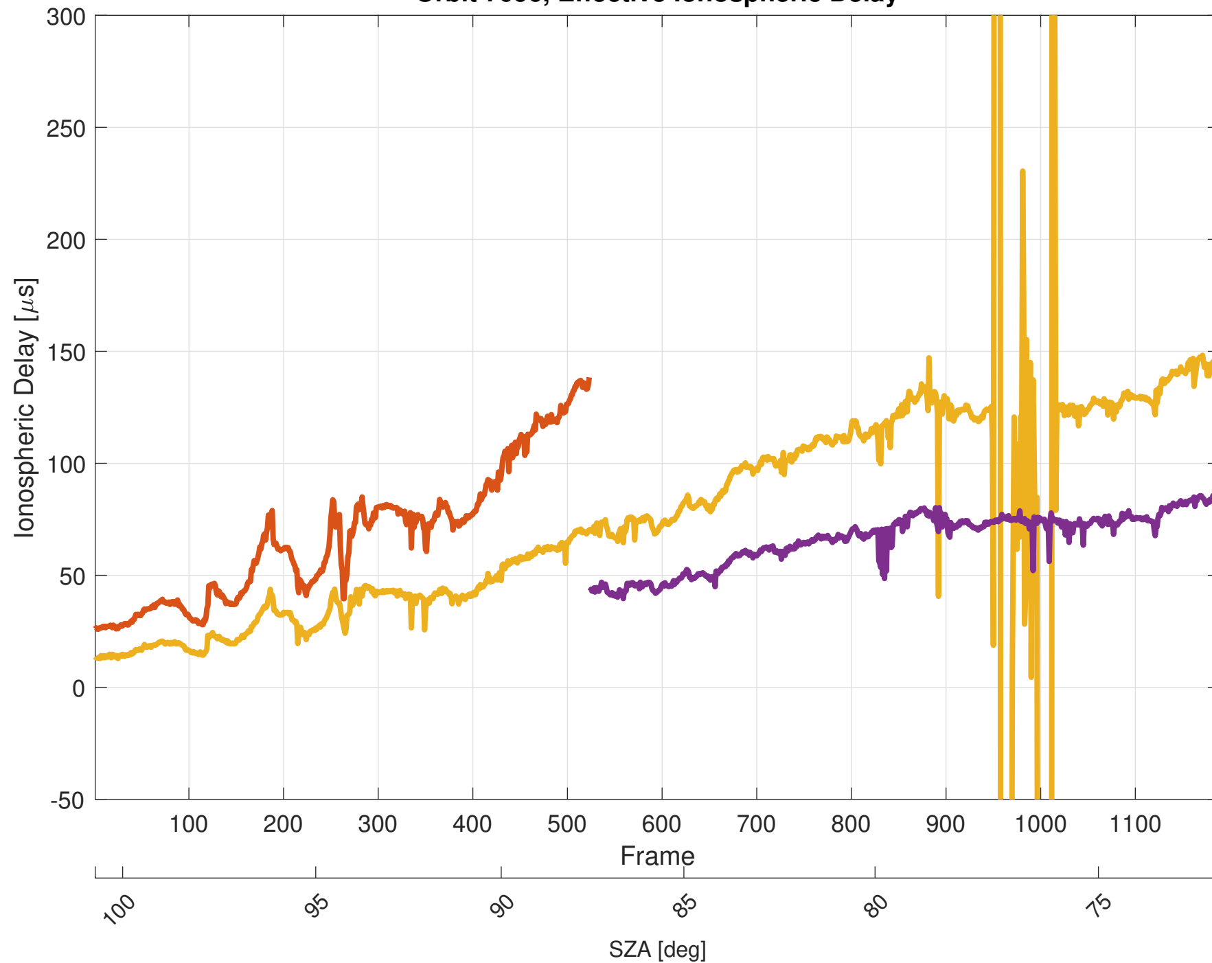
Orbit 7096, Effective Ionospheric Delay
