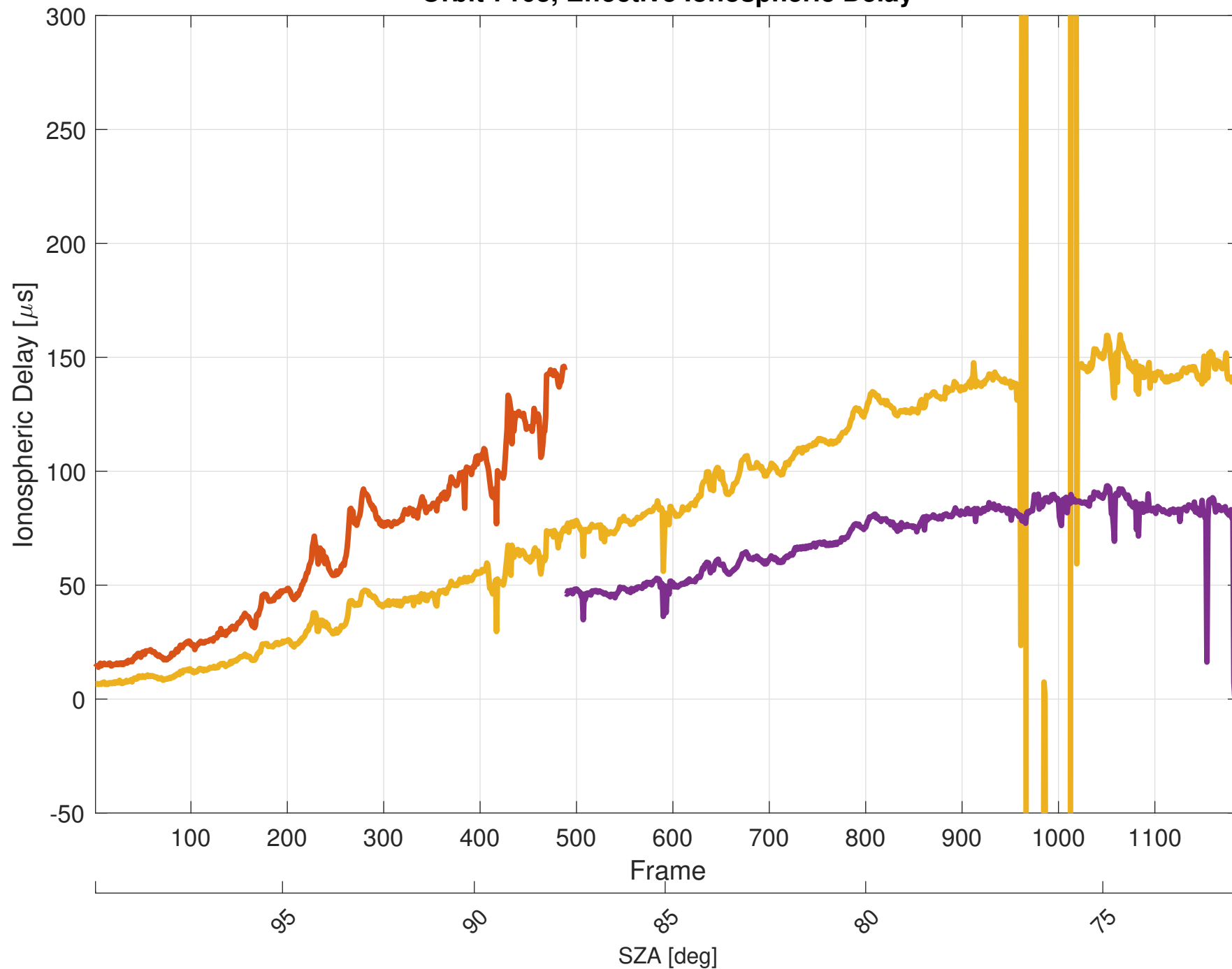
Orbit 7103, Effective Ionospheric Delay
