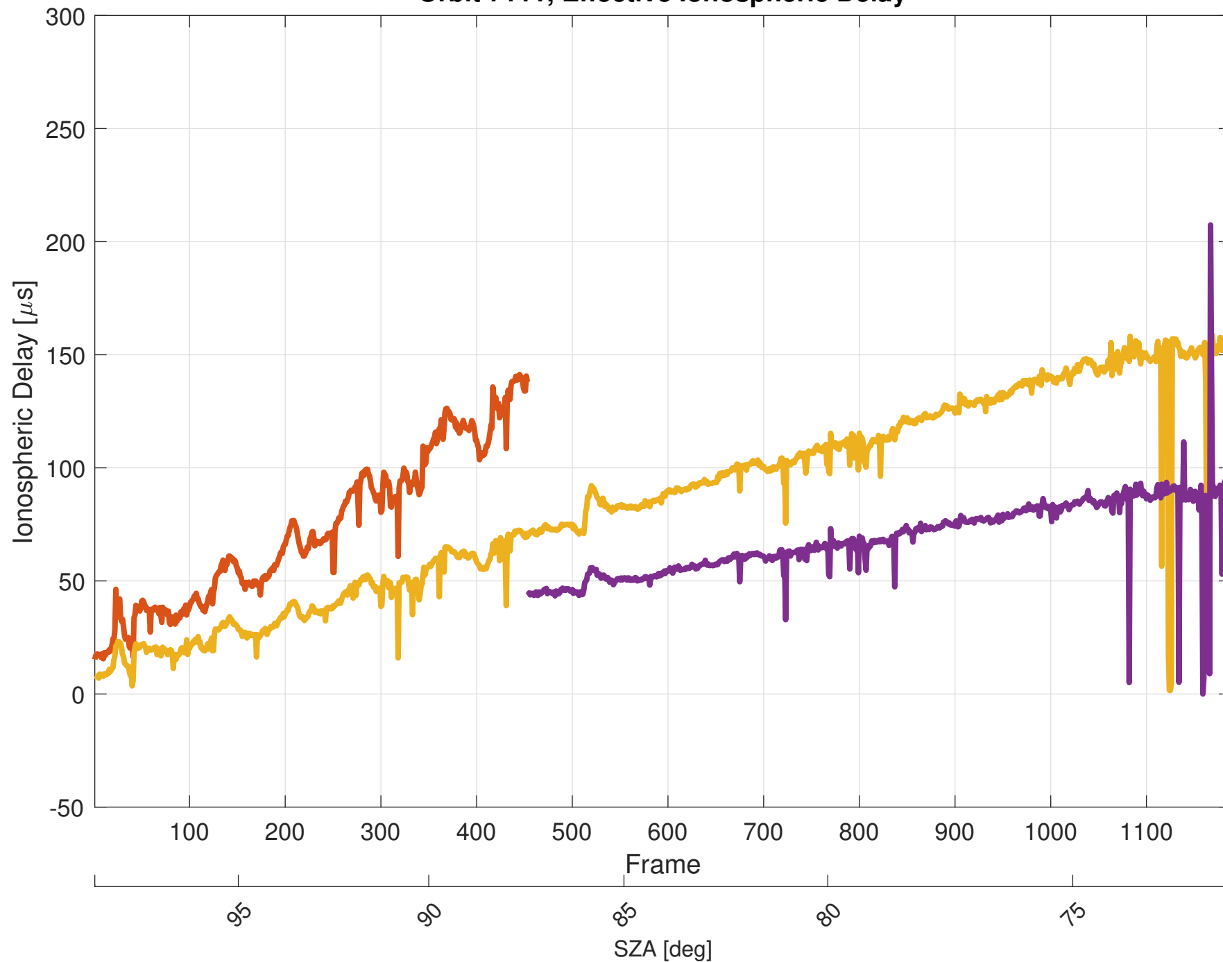
Orbit 7111, Effective Ionospheric Delay
