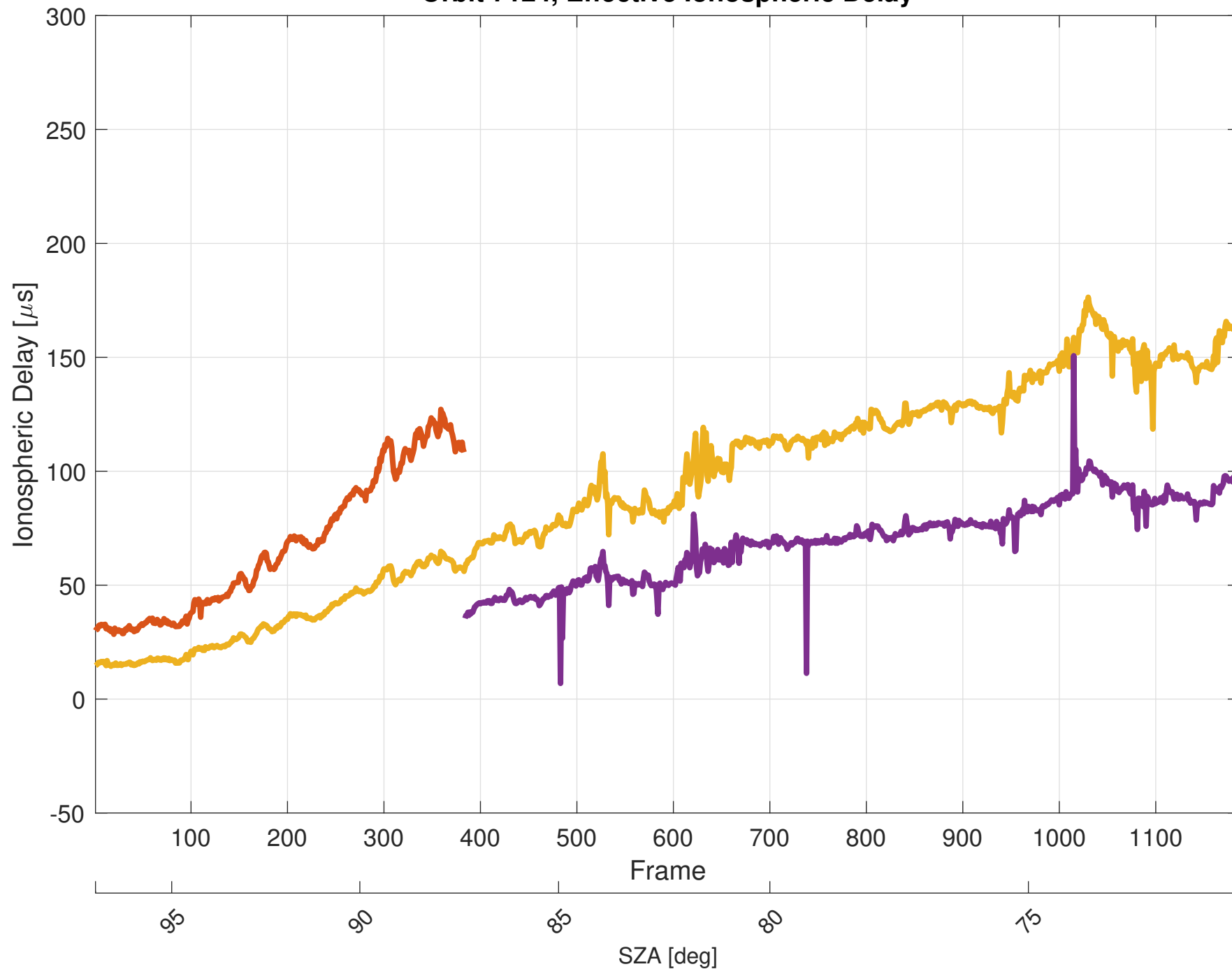
Orbit 7124, Effective Ionospheric Delay
