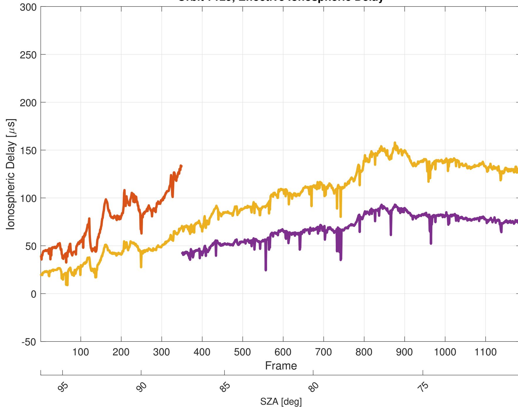
Orbit 7129, Effective Ionospheric Delay
