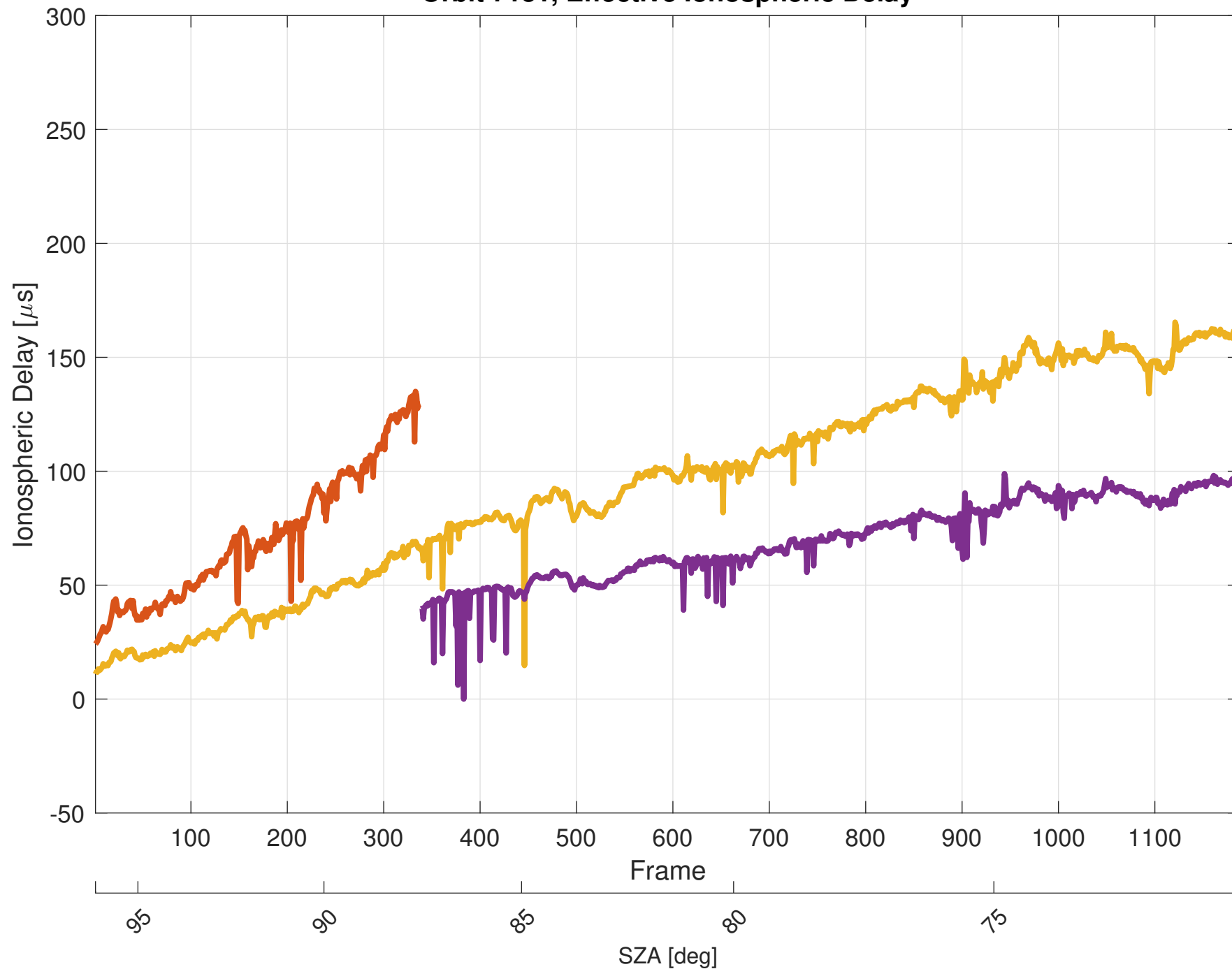
Orbit 7131, Effective Ionospheric Delay
