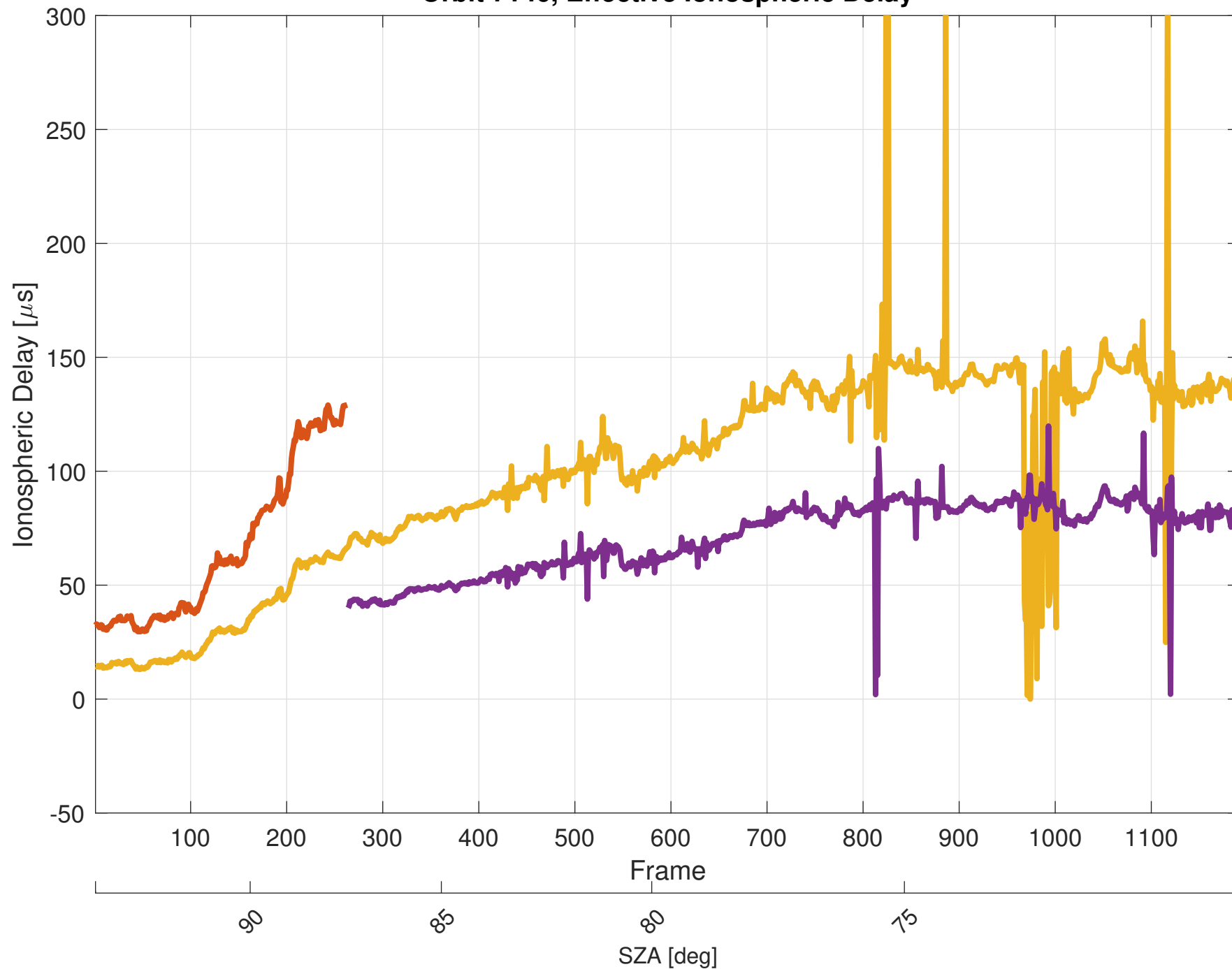
Orbit 7146, Effective Ionospheric Delay
