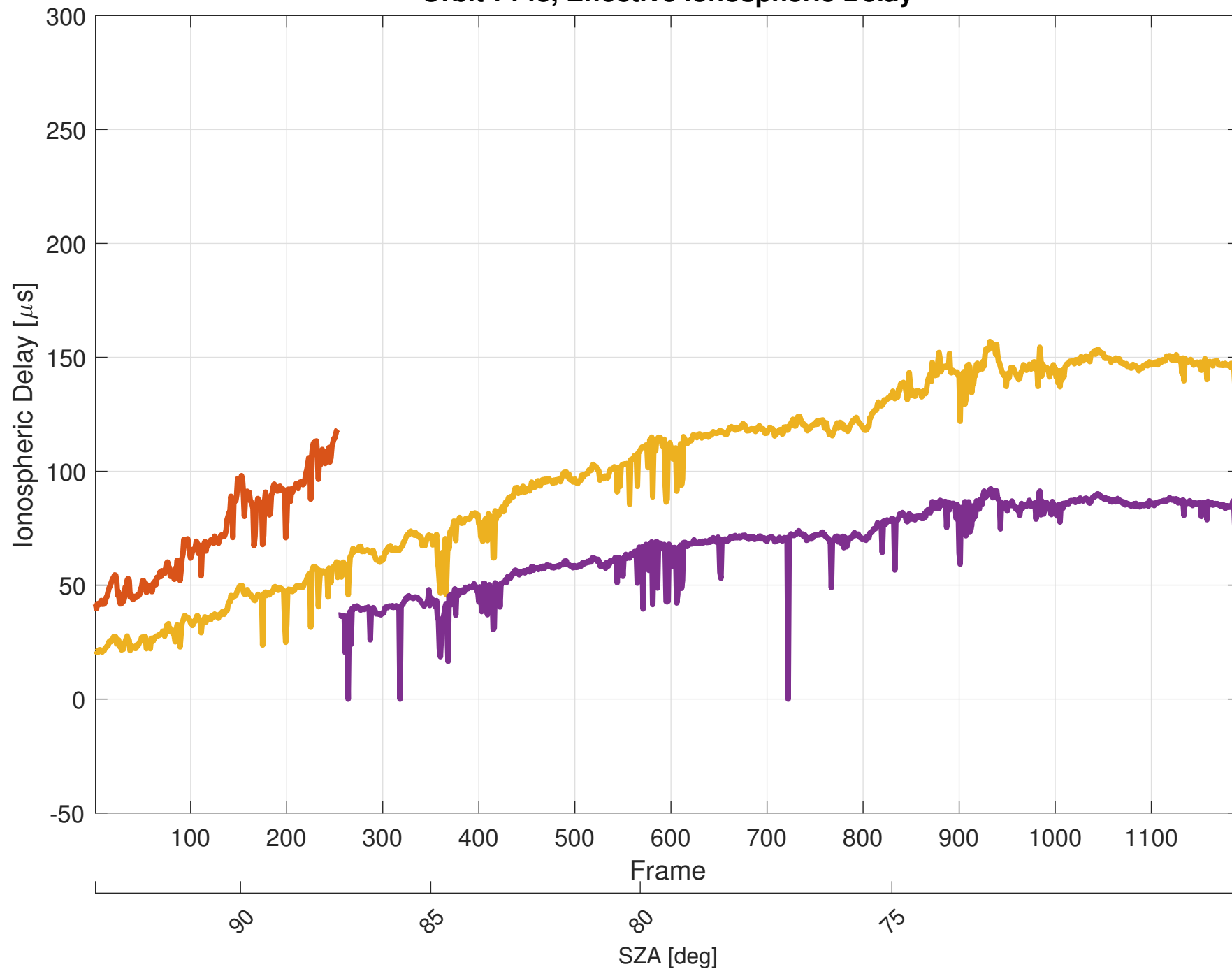
Orbit 7148, Effective Ionospheric Delay
