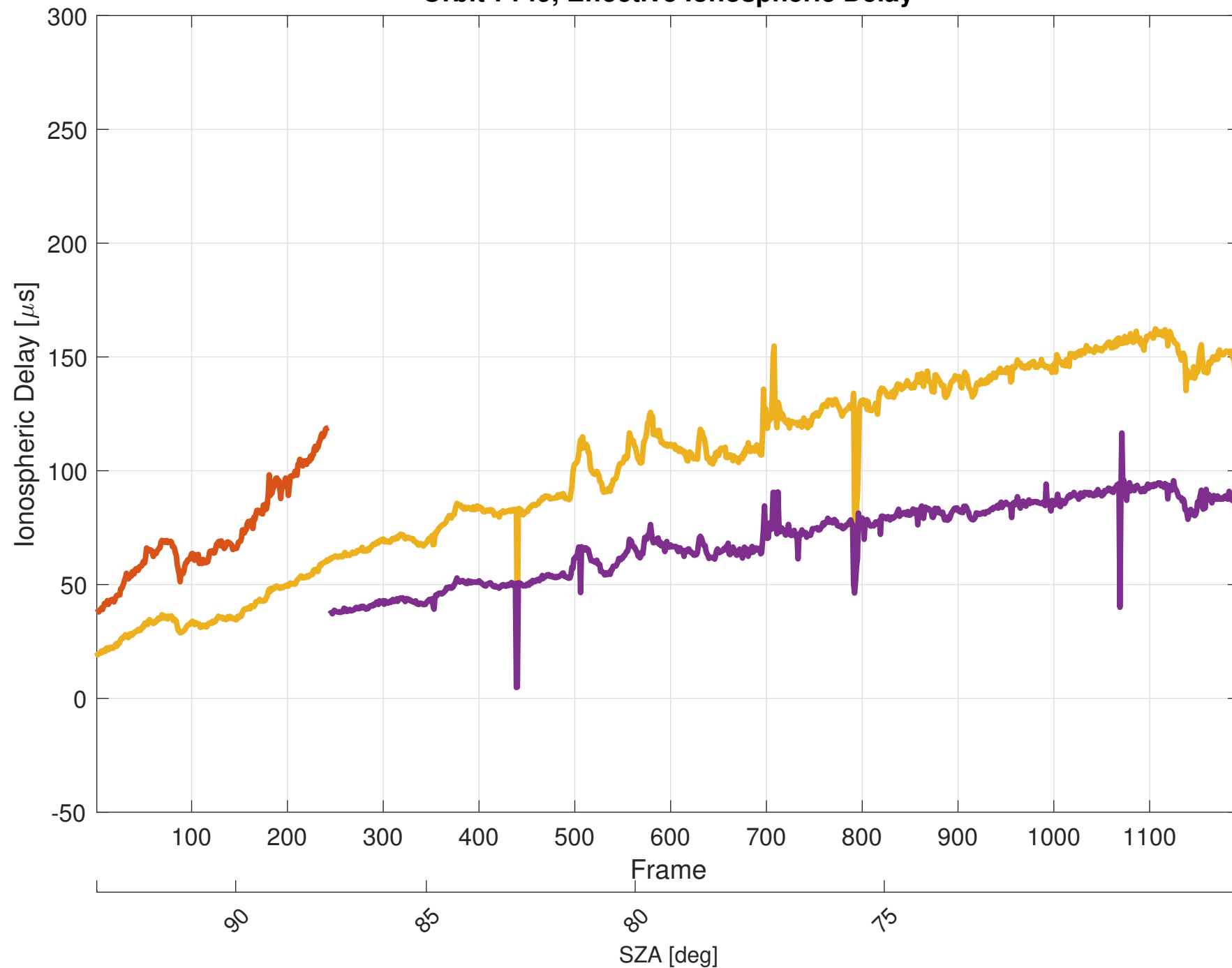
Orbit 7149, Effective Ionospheric Delay
