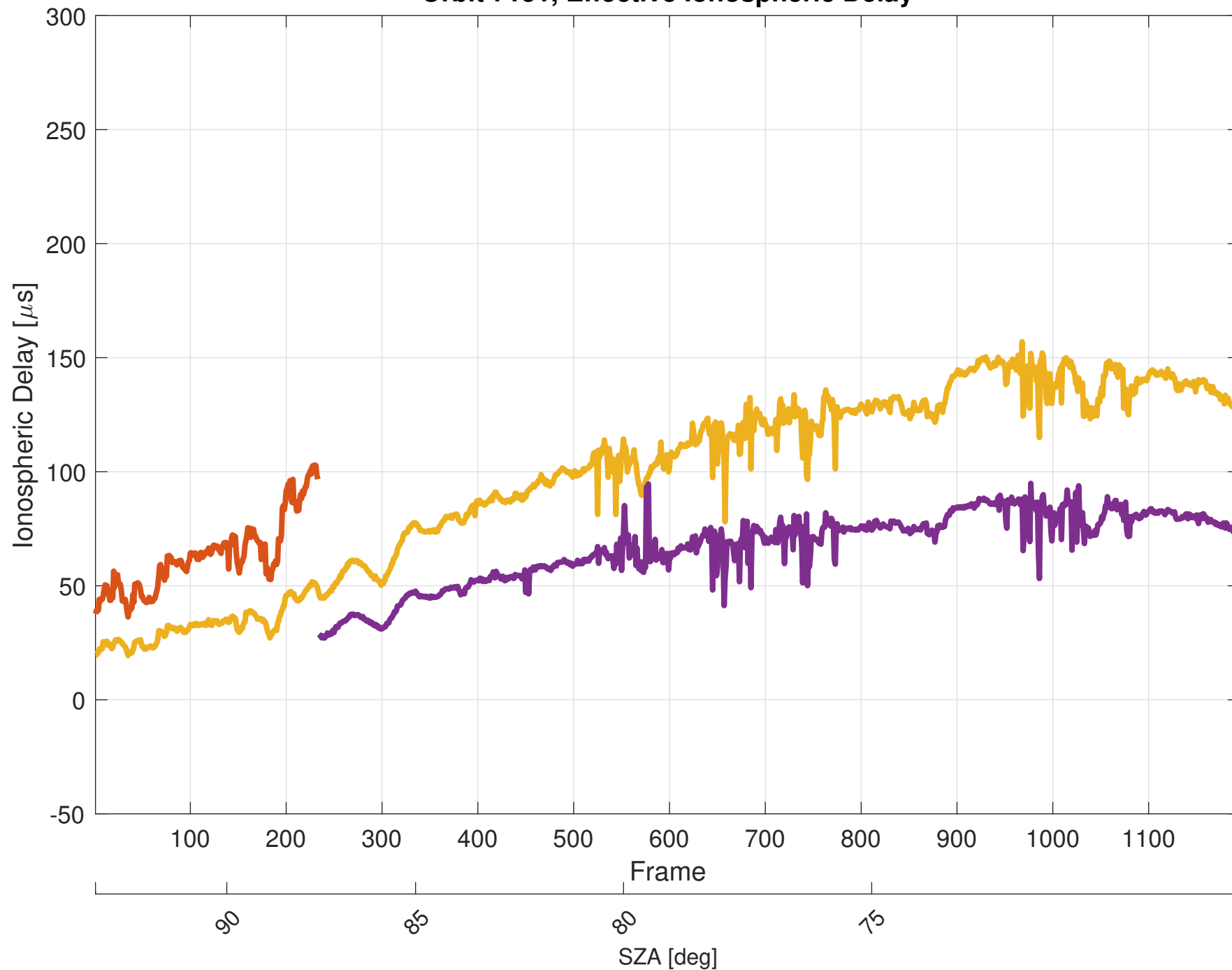
Orbit 7151, Effective Ionospheric Delay
