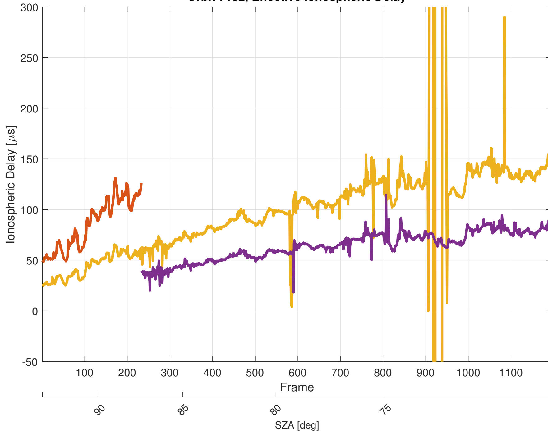
Orbit 7152, Effective Ionospheric Delay
