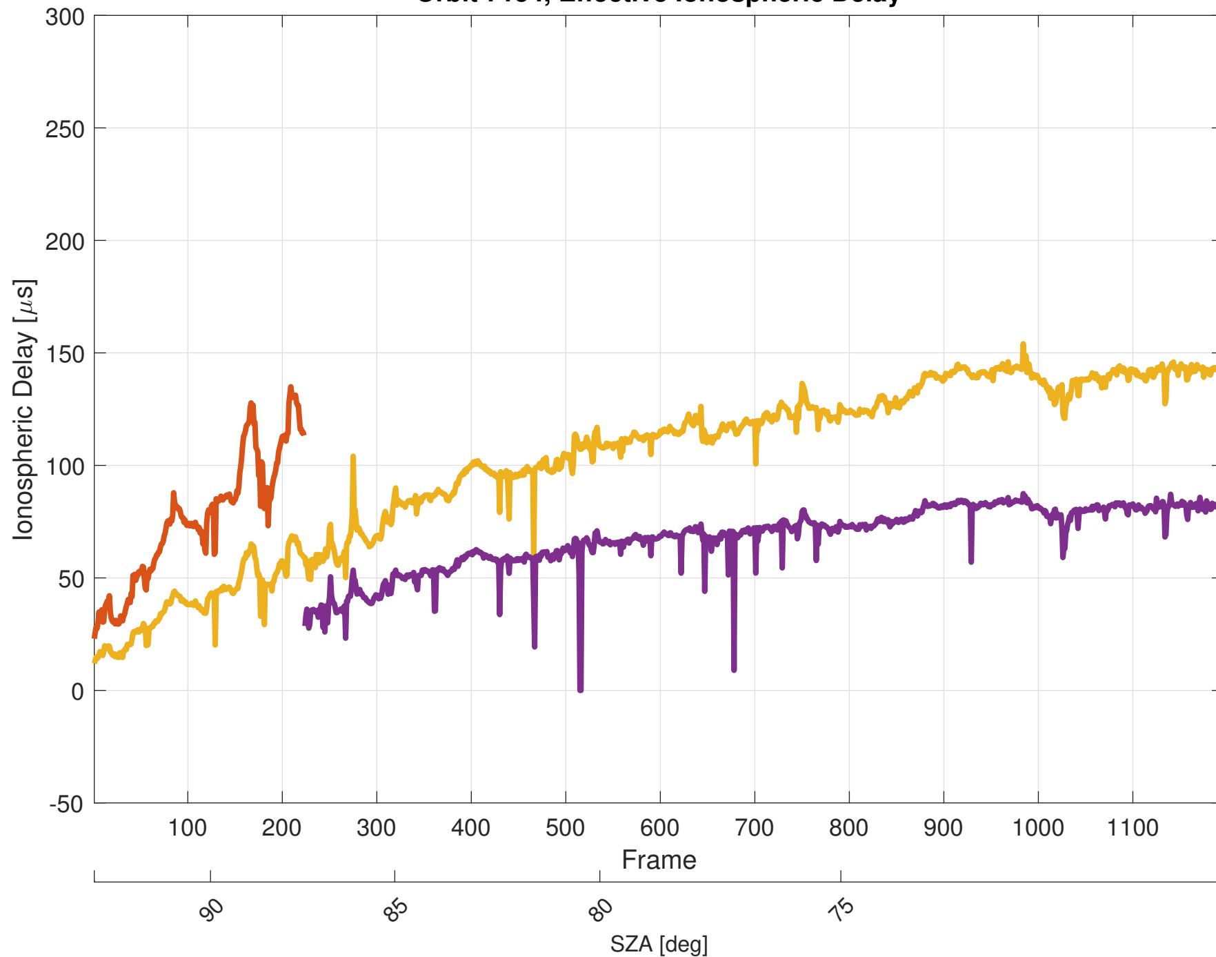
Orbit 7154, Effective Ionospheric Delay
