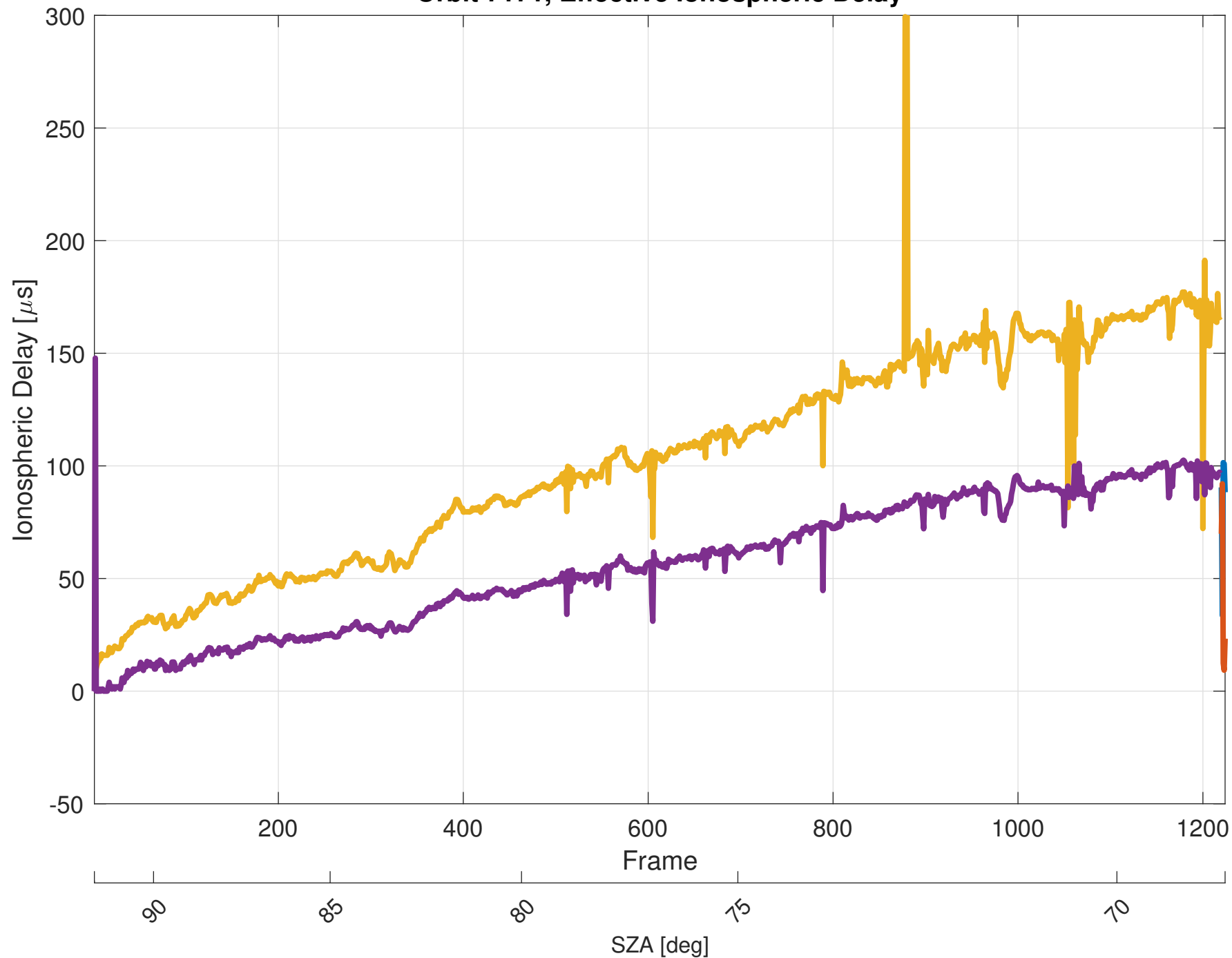
Orbit 7171, Effective Ionospheric Delay
