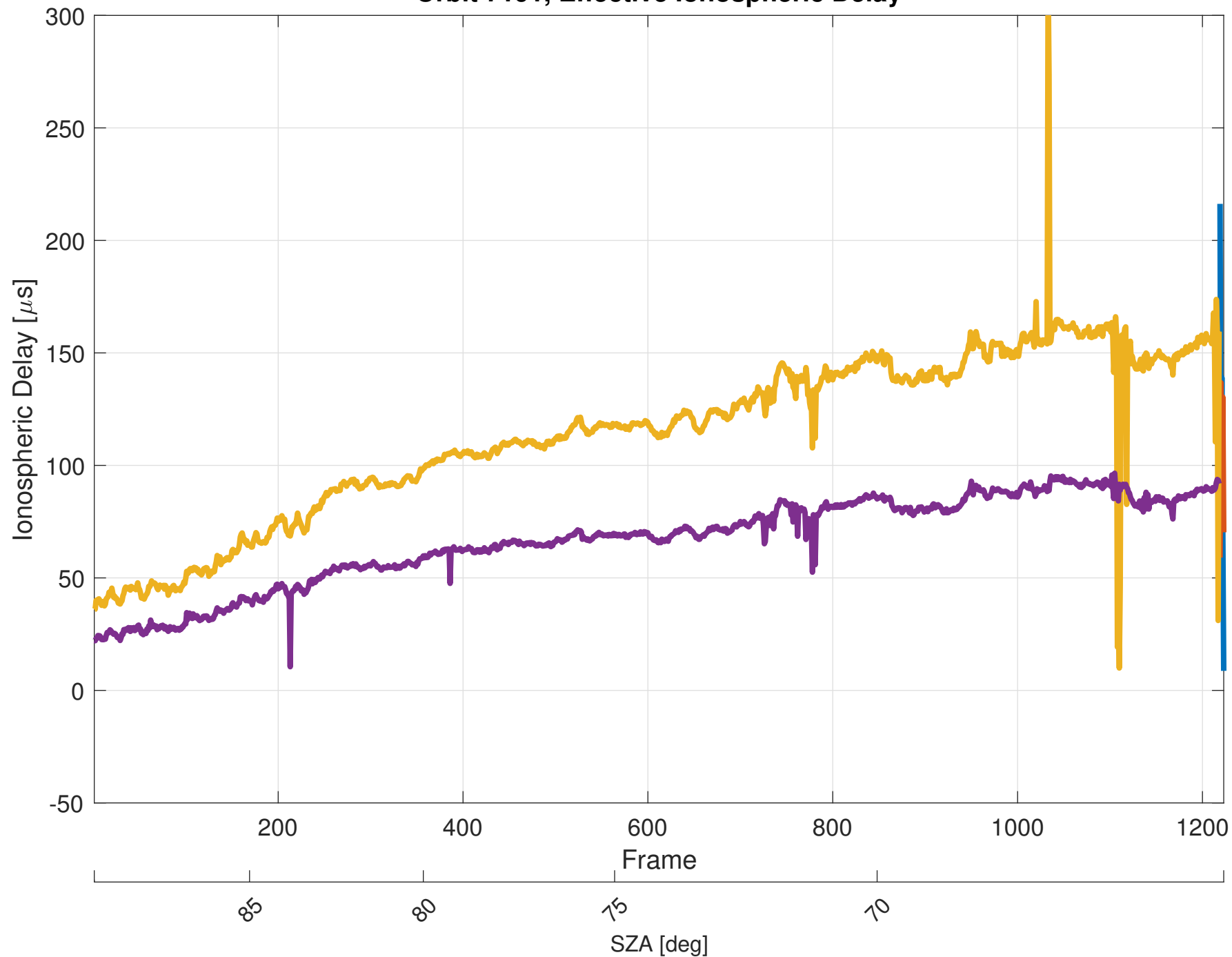
Orbit 7191, Effective Ionospheric Delay
