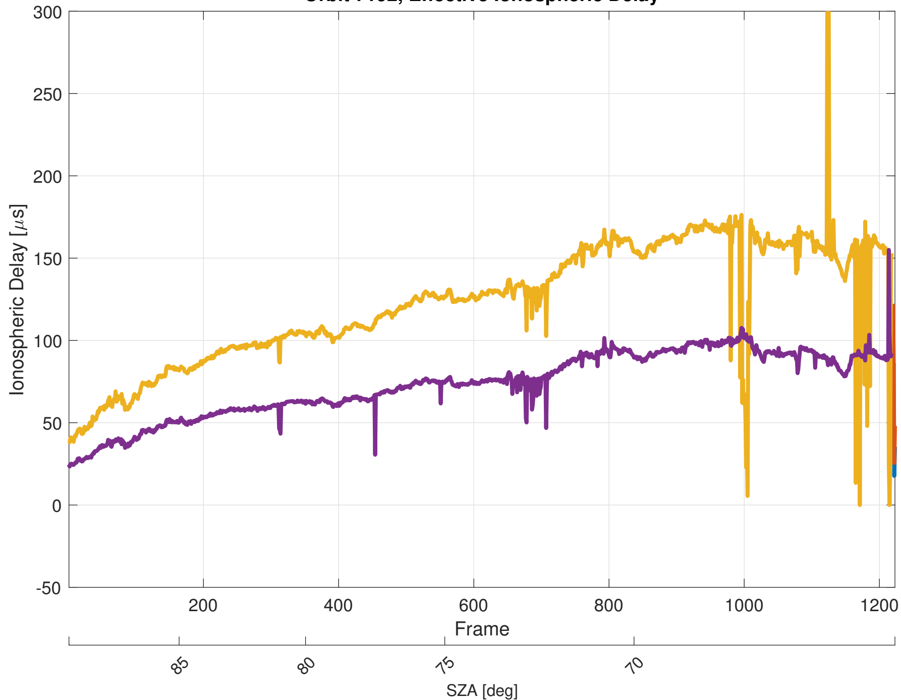
Orbit 7192, Effective Ionospheric Delay
