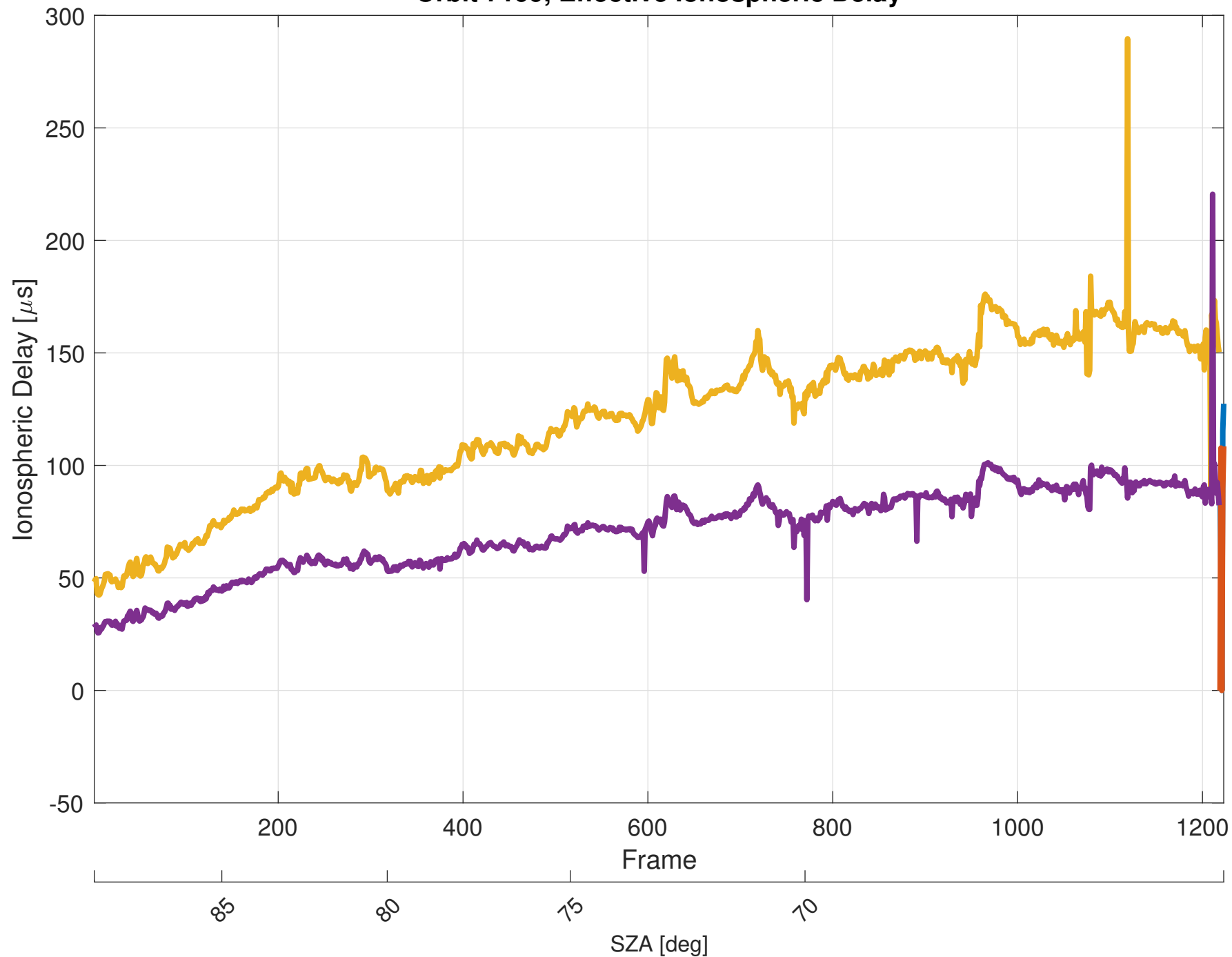
Orbit 7199, Effective Ionospheric Delay
