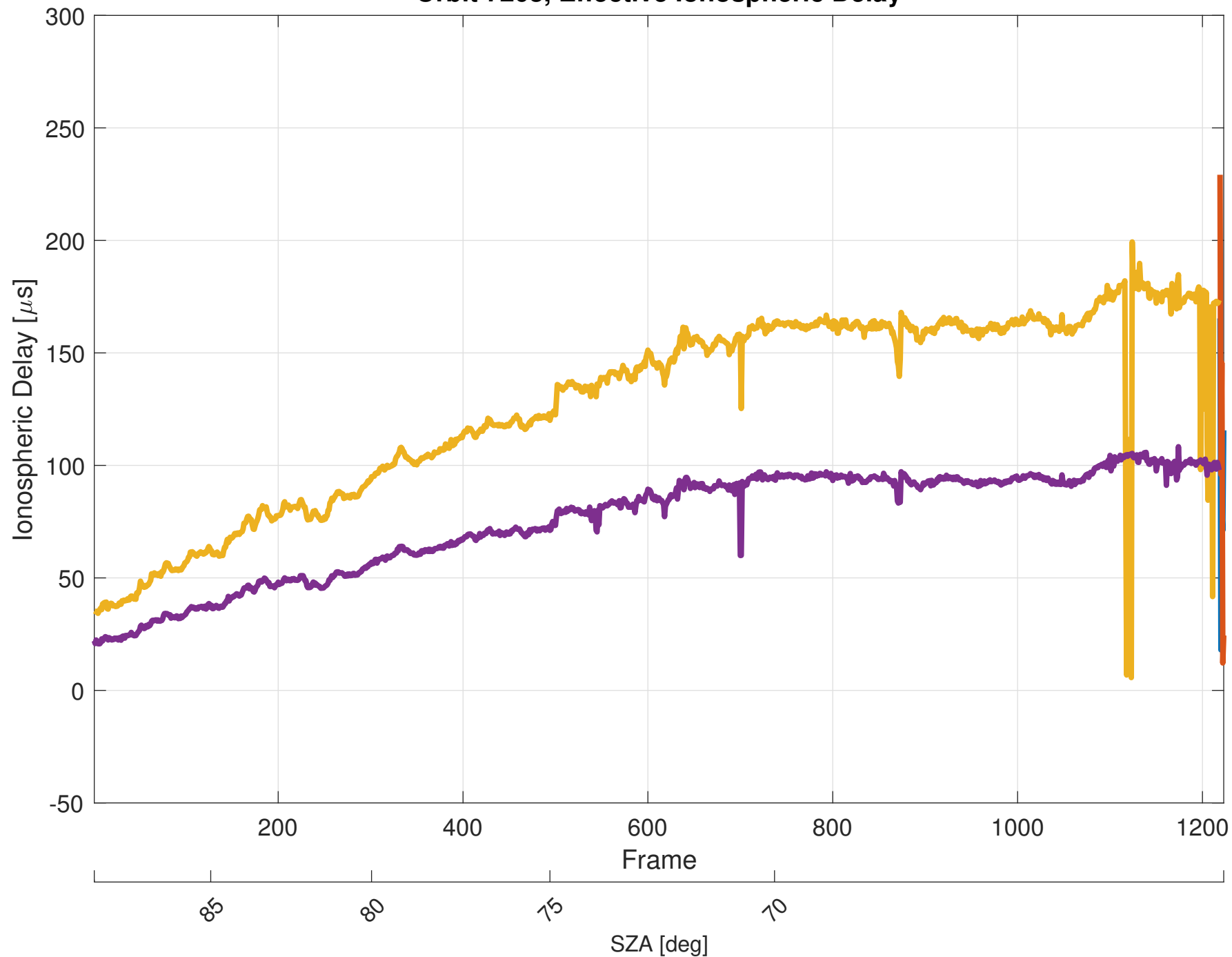
Orbit 7203, Effective Ionospheric Delay
