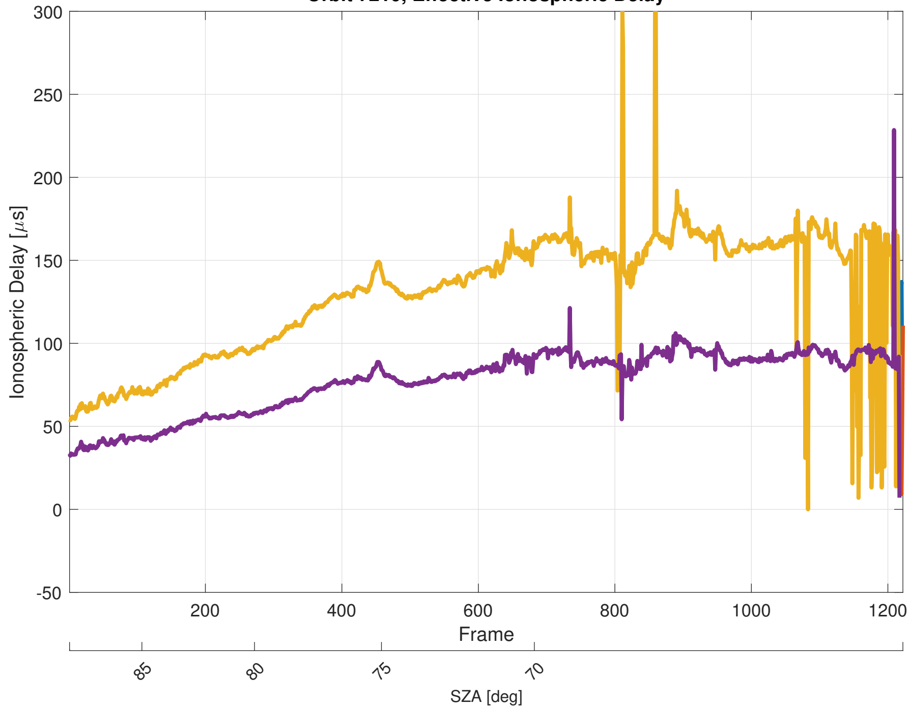
Orbit 7210, Effective Ionospheric Delay
