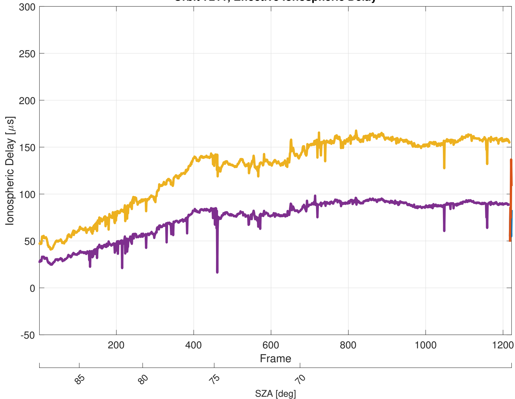
Orbit 7211, Effective Ionospheric Delay
