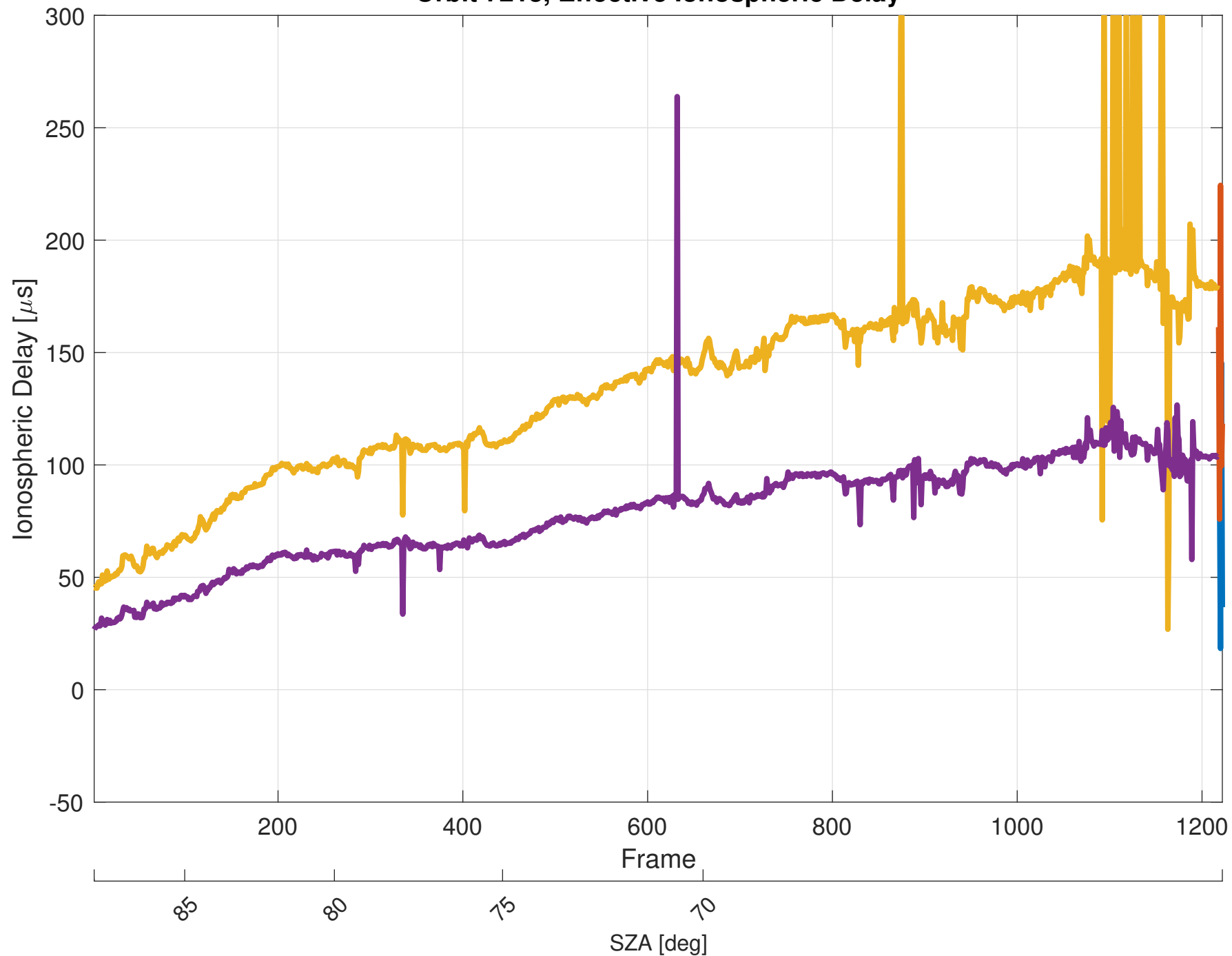
Orbit 7213, Effective Ionospheric Delay
