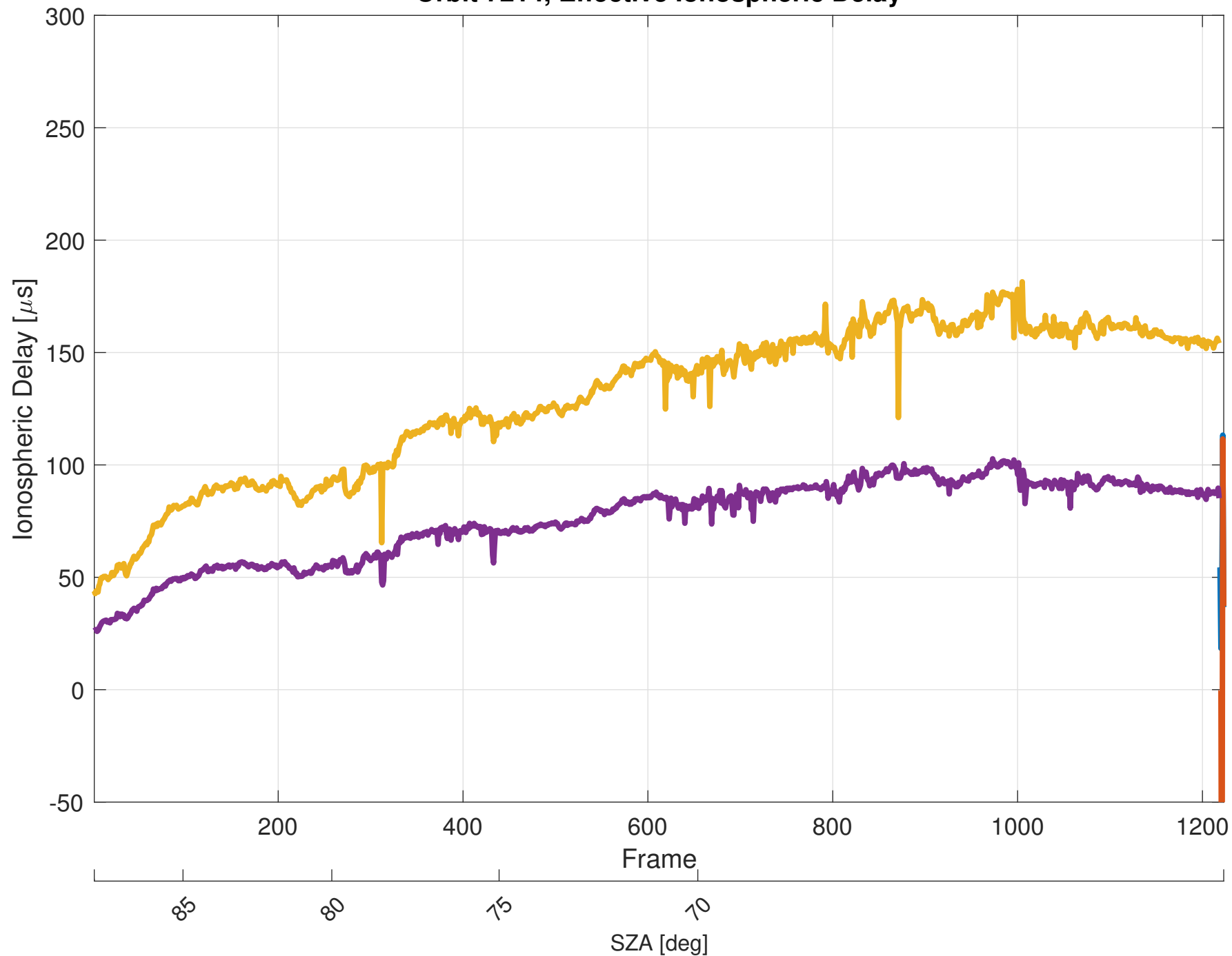
Orbit 7214, Effective Ionospheric Delay
