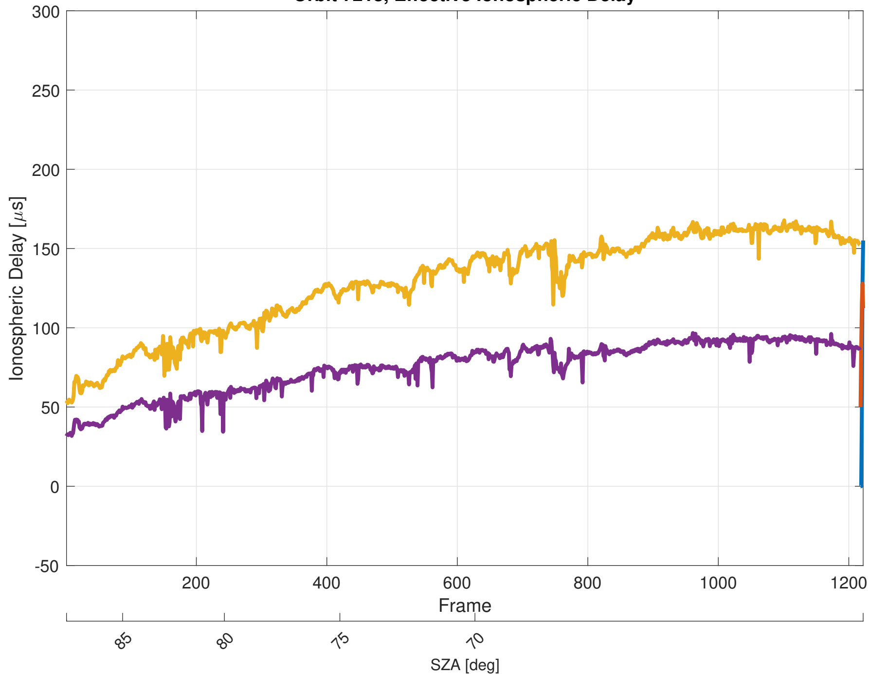
Orbit 7218, Effective Ionospheric Delay
