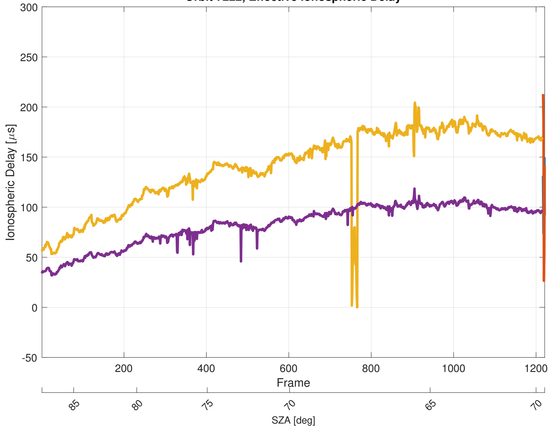
Orbit 7222, Effective Ionospheric Delay
