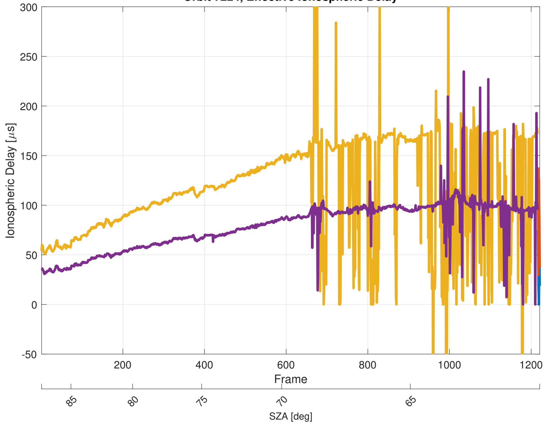
Orbit 7224, Effective Ionospheric Delay
