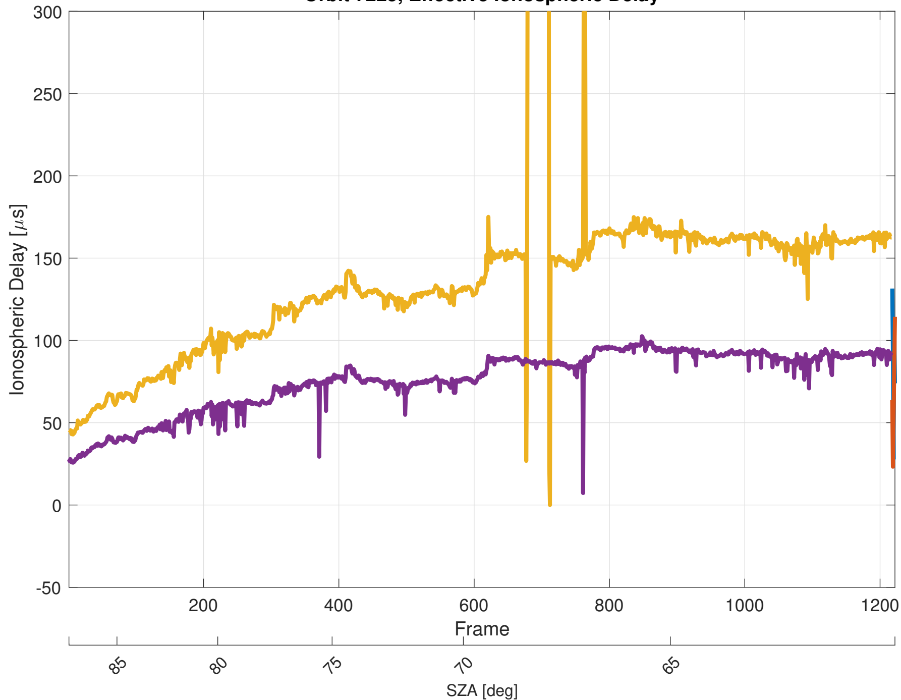
Orbit 7225, Effective Ionospheric Delay
