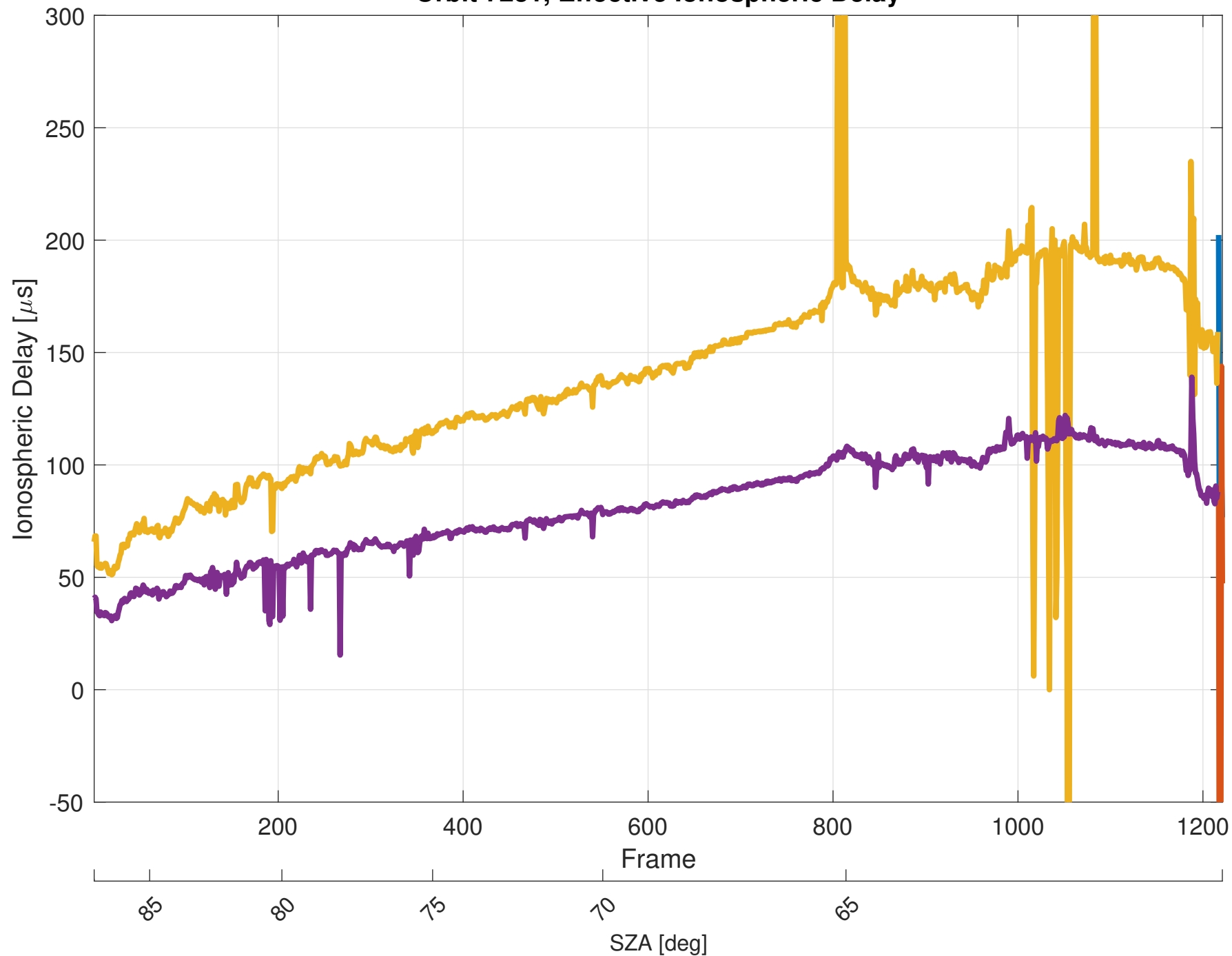
Orbit 7231, Effective Ionospheric Delay
