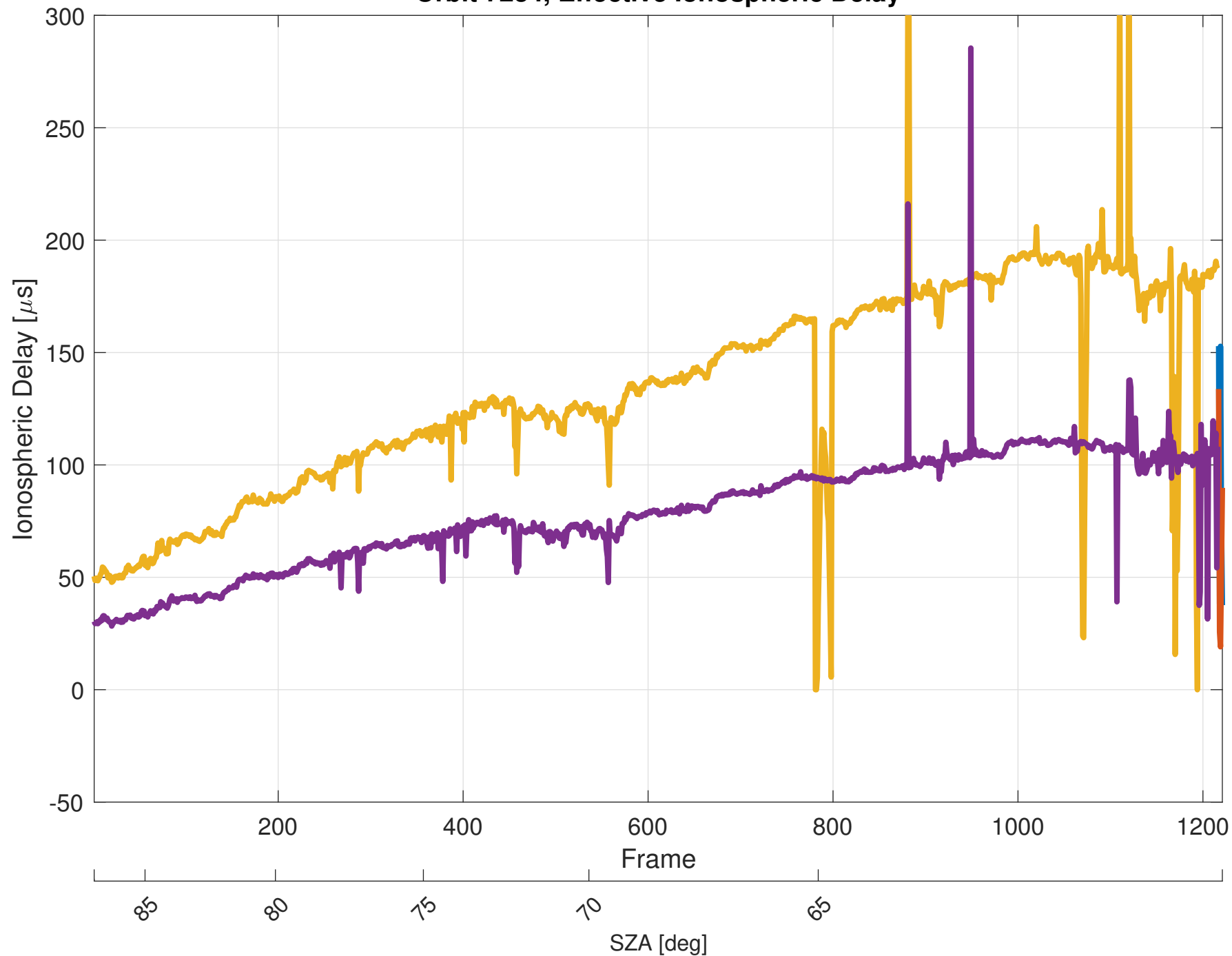
Orbit 7234, Effective Ionospheric Delay
