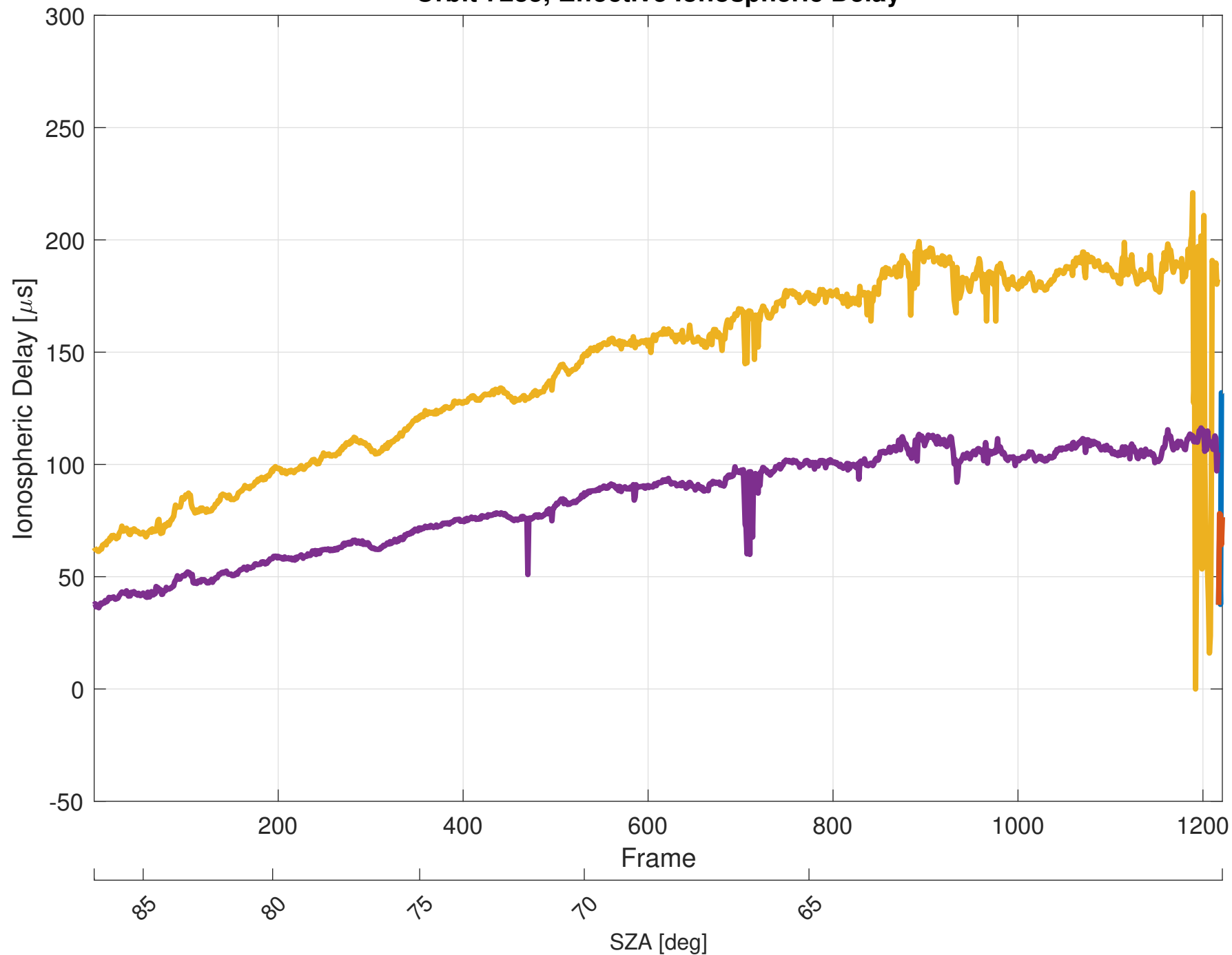
Orbit 7235, Effective Ionospheric Delay
