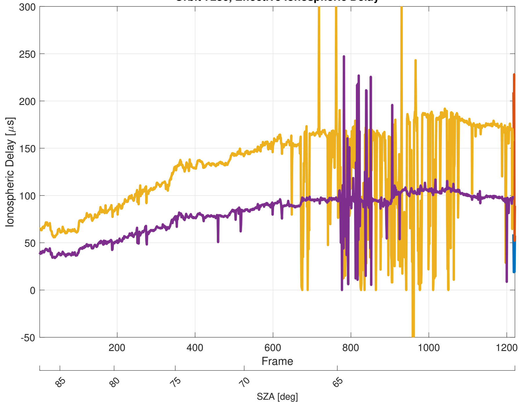
Orbit 7236, Effective Ionospheric Delay
